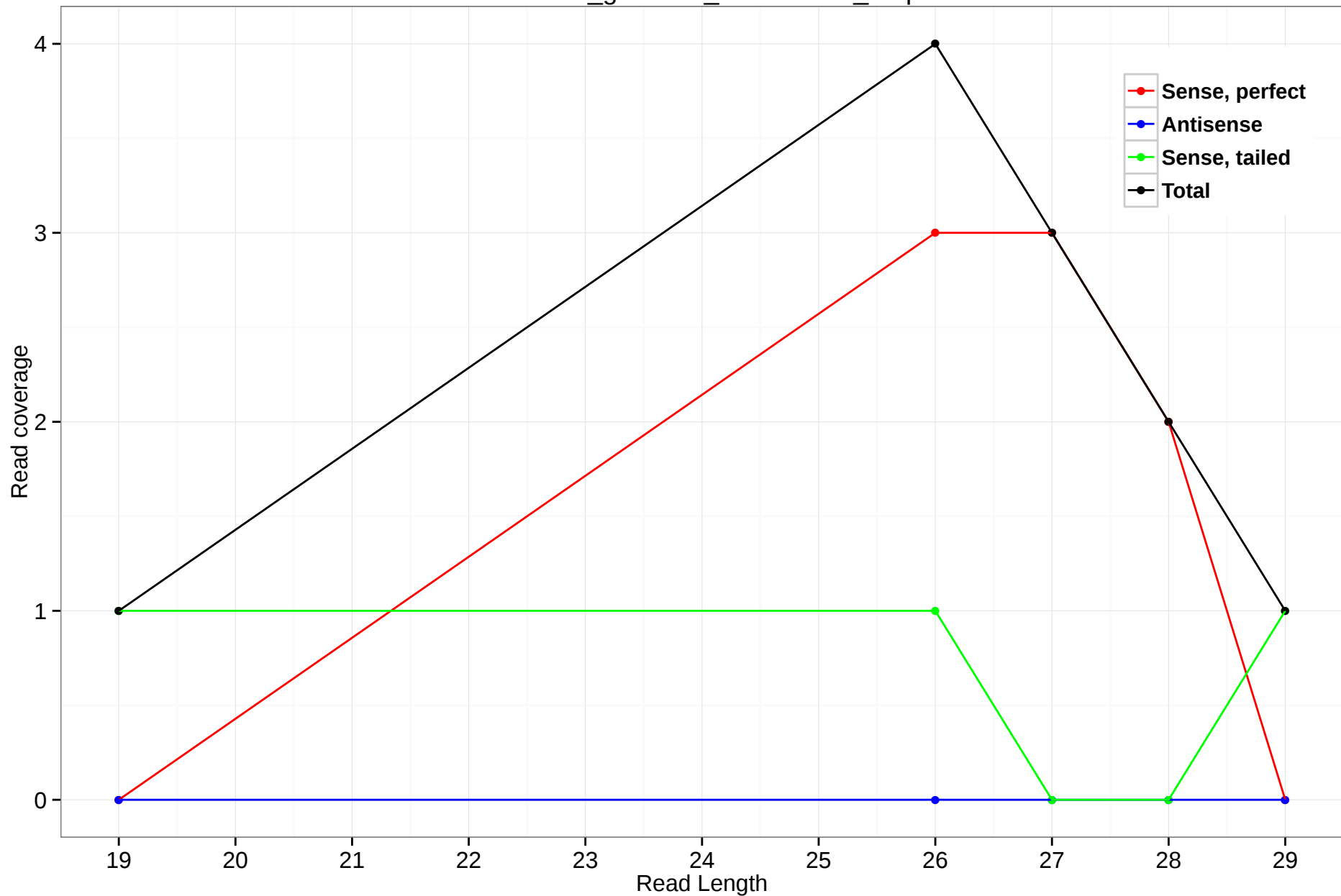
rheMac3_genscan_chr10.1464_1.5p
