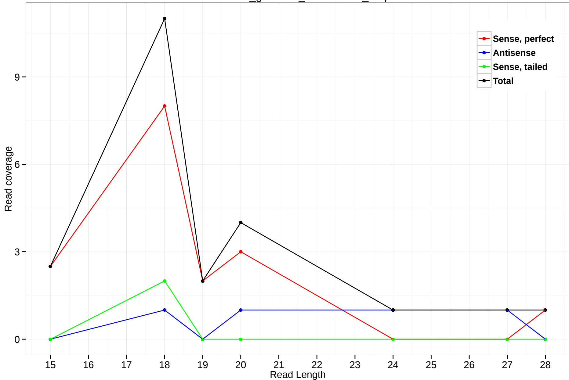
rheMac3_genscan_chr10.1455_0.5p
