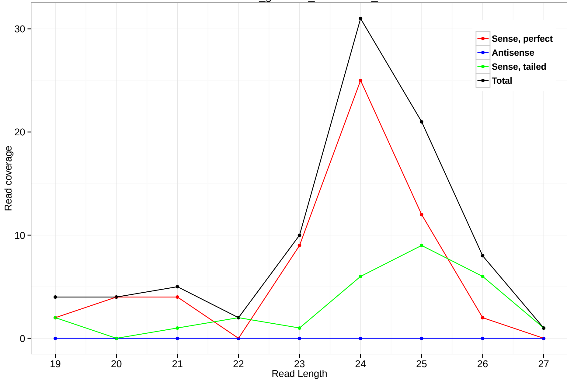
rheMac3_genscan_chr10.1442_5
