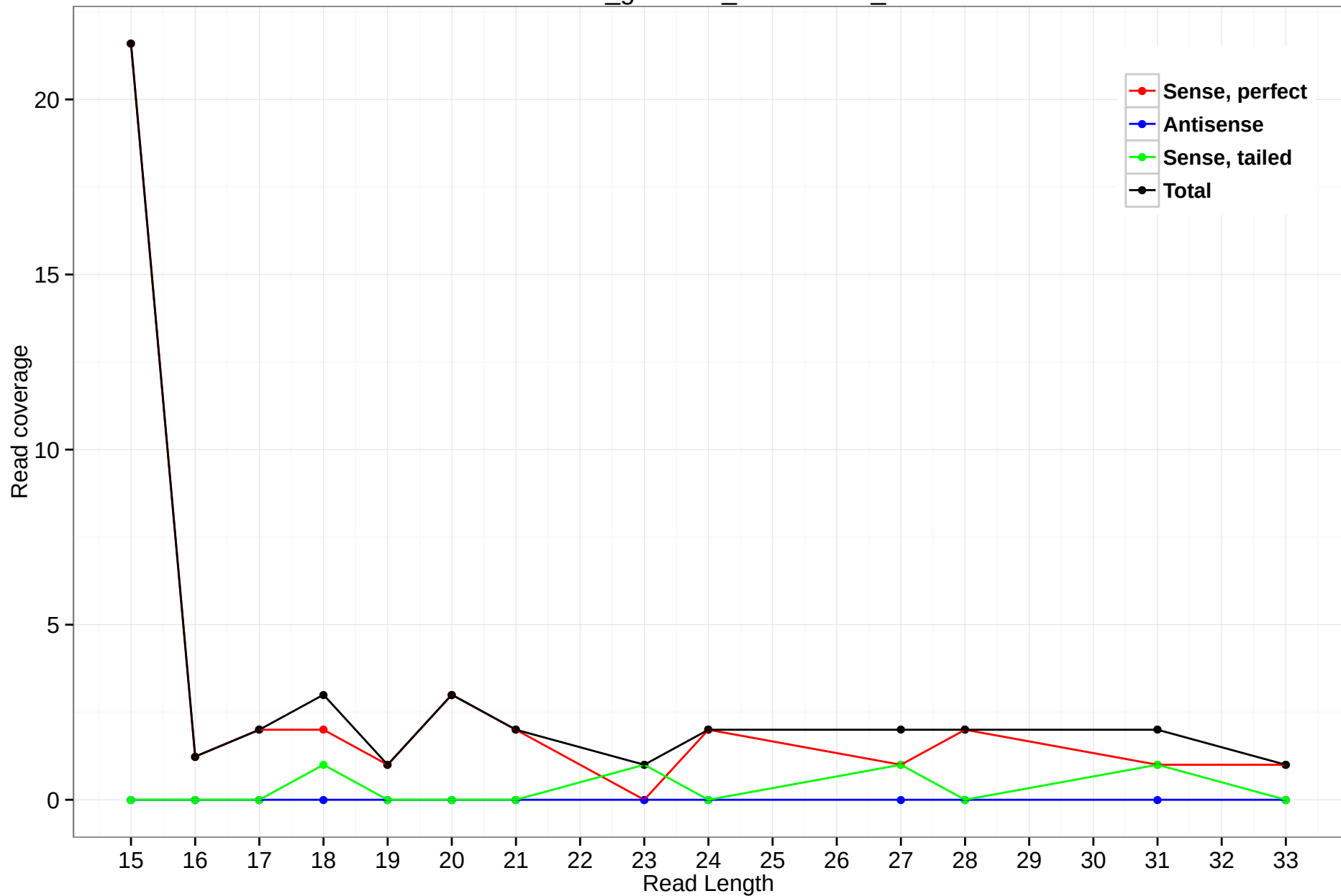
rheMac3_genscan_chr10.1430_11
