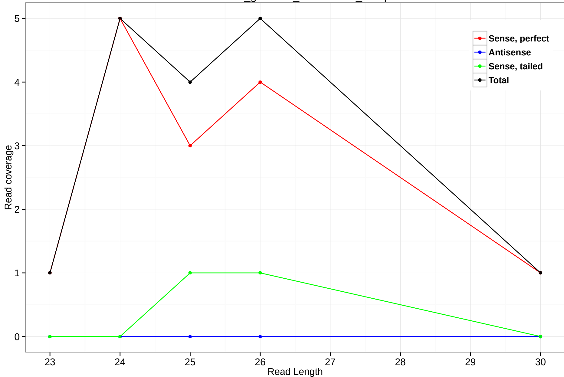
rheMac3_genscan_chr10.1386_48.5p
