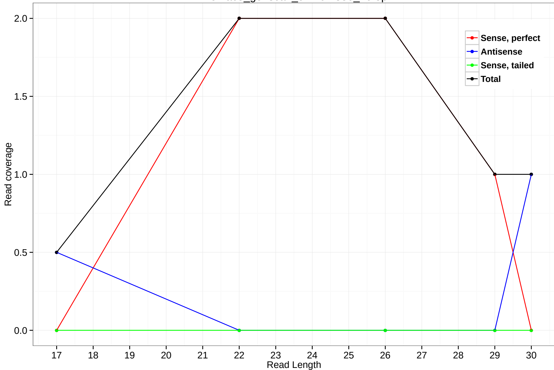
rheMac3_genscan_chr10.1386_40.5p
