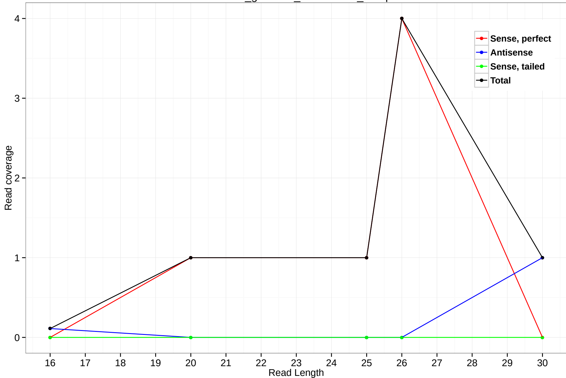
rheMac3_genscan_chr10.1386_36.3p
