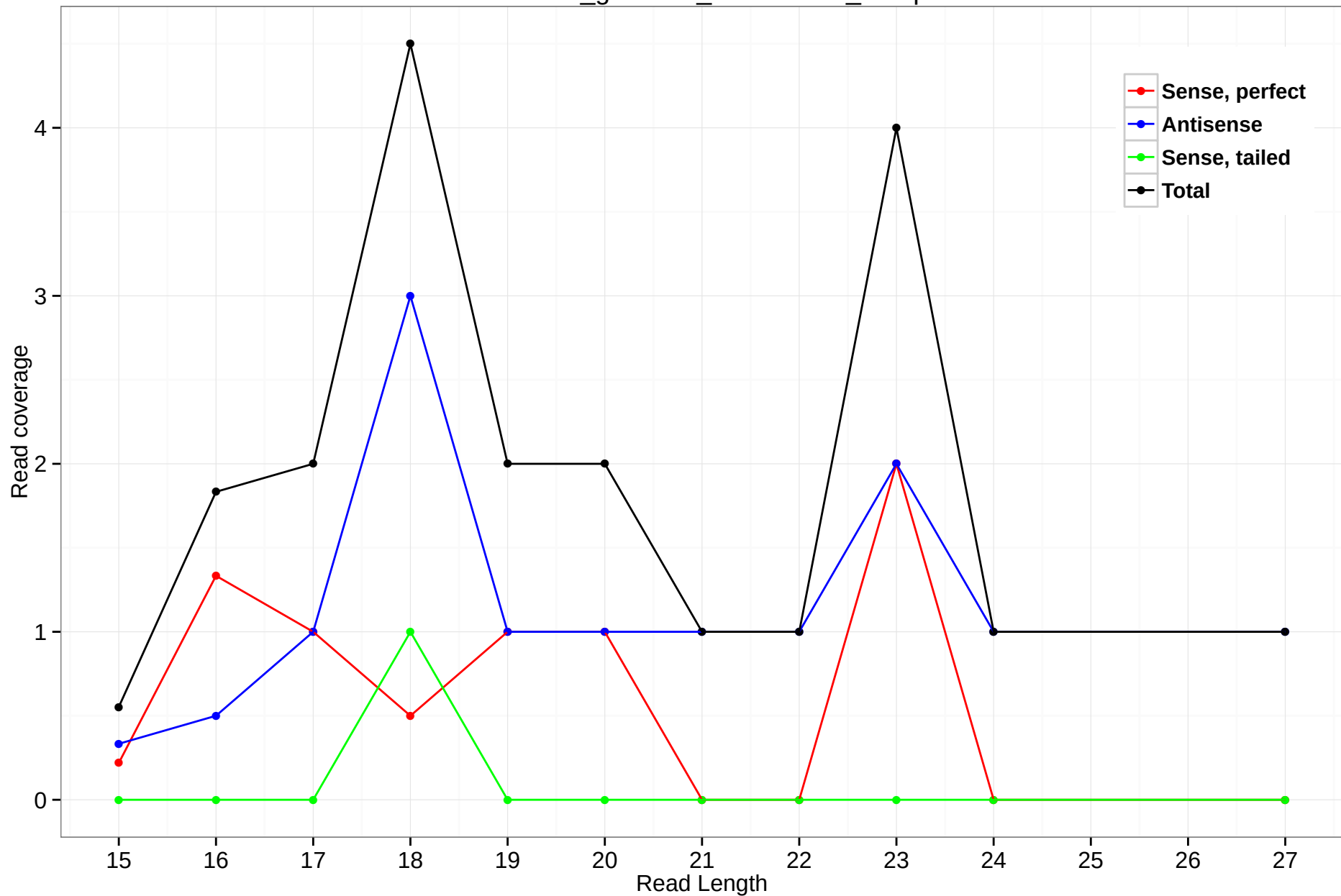
rheMac3_genscan_chr10.1377_10.3p
