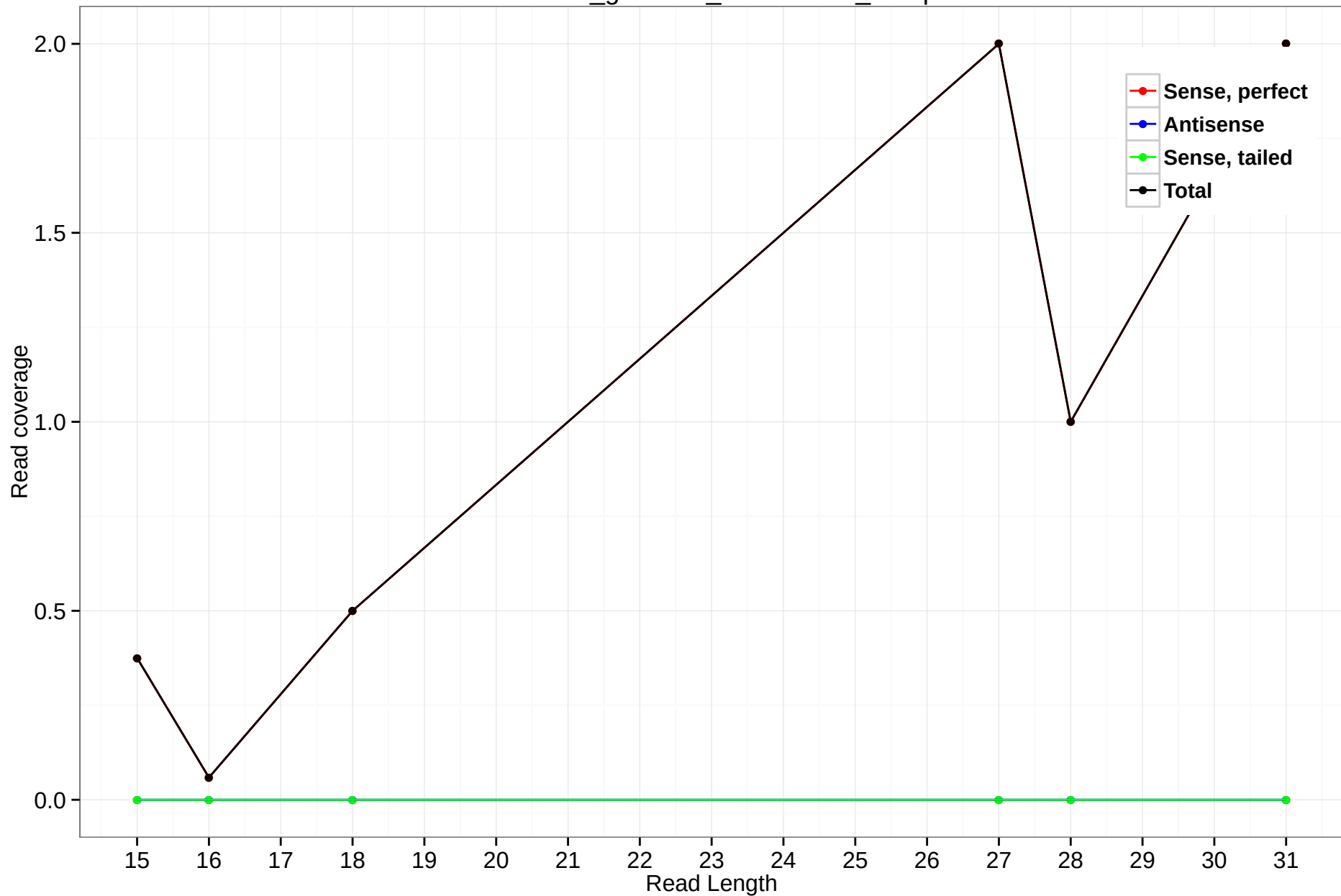
rheMac3_genscan_chr10.1366_15.5p
