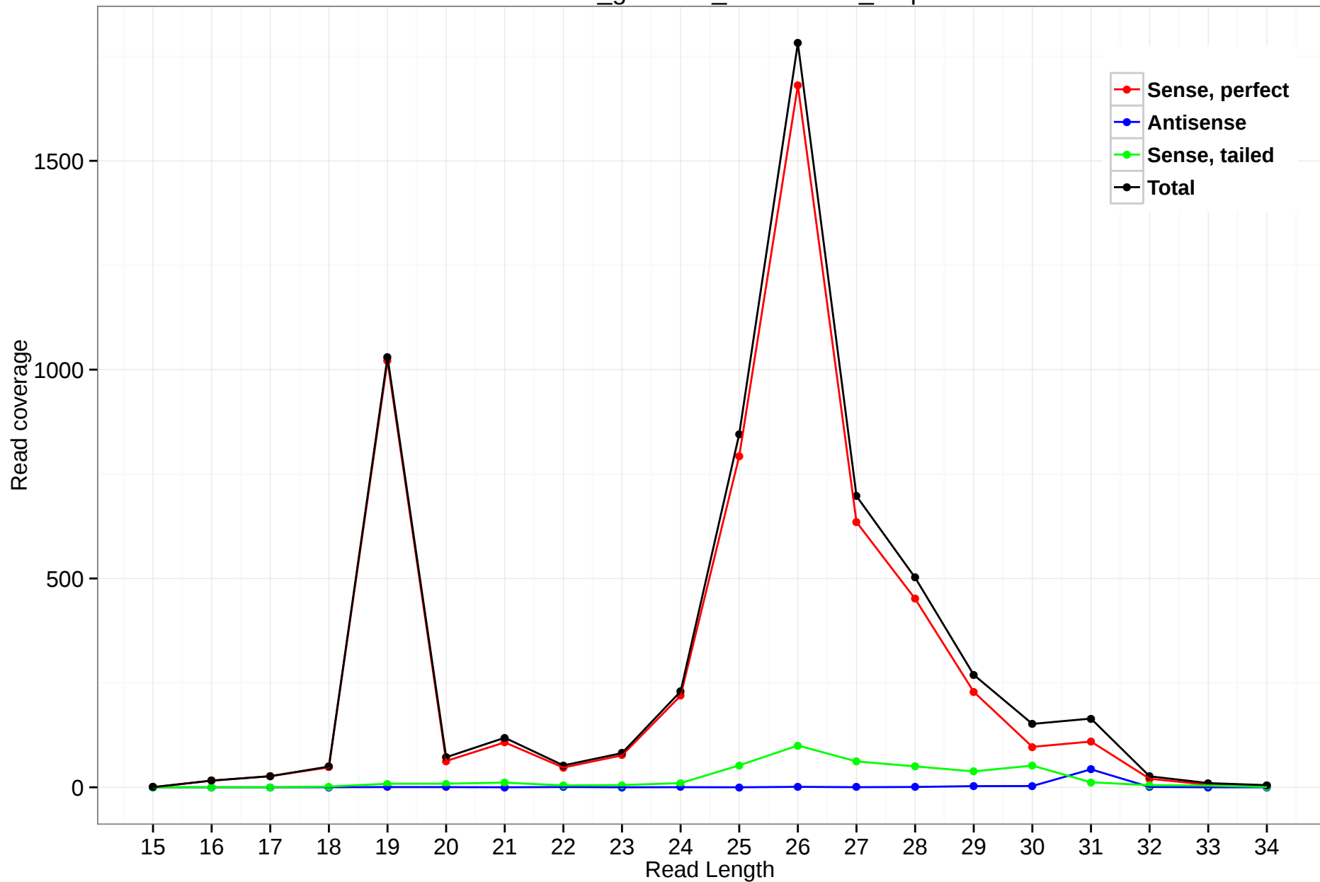
rheMac3_genscan_chr10.1357_5.5p
