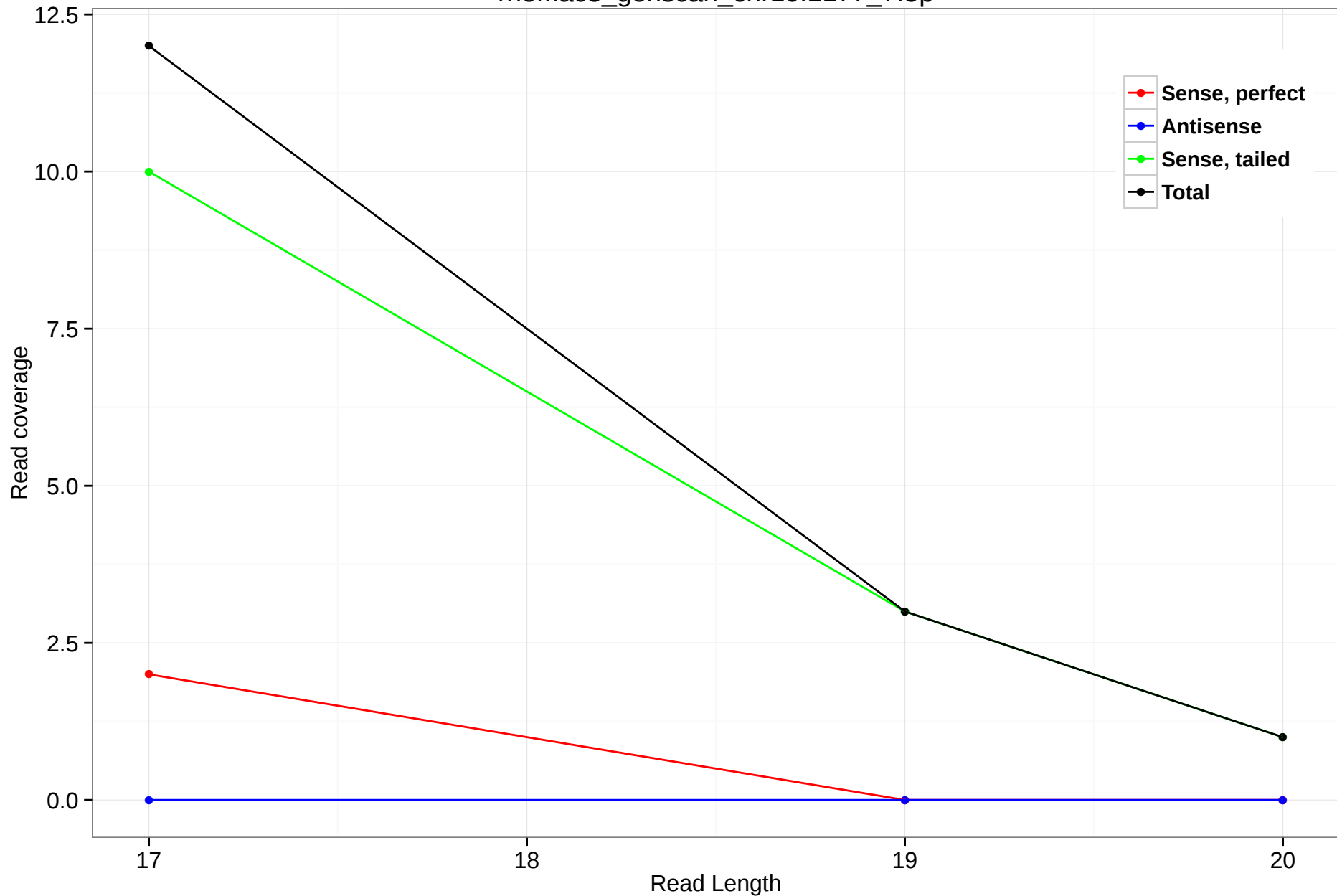
rheMac3_genscan_chr10.1177_7.5p
