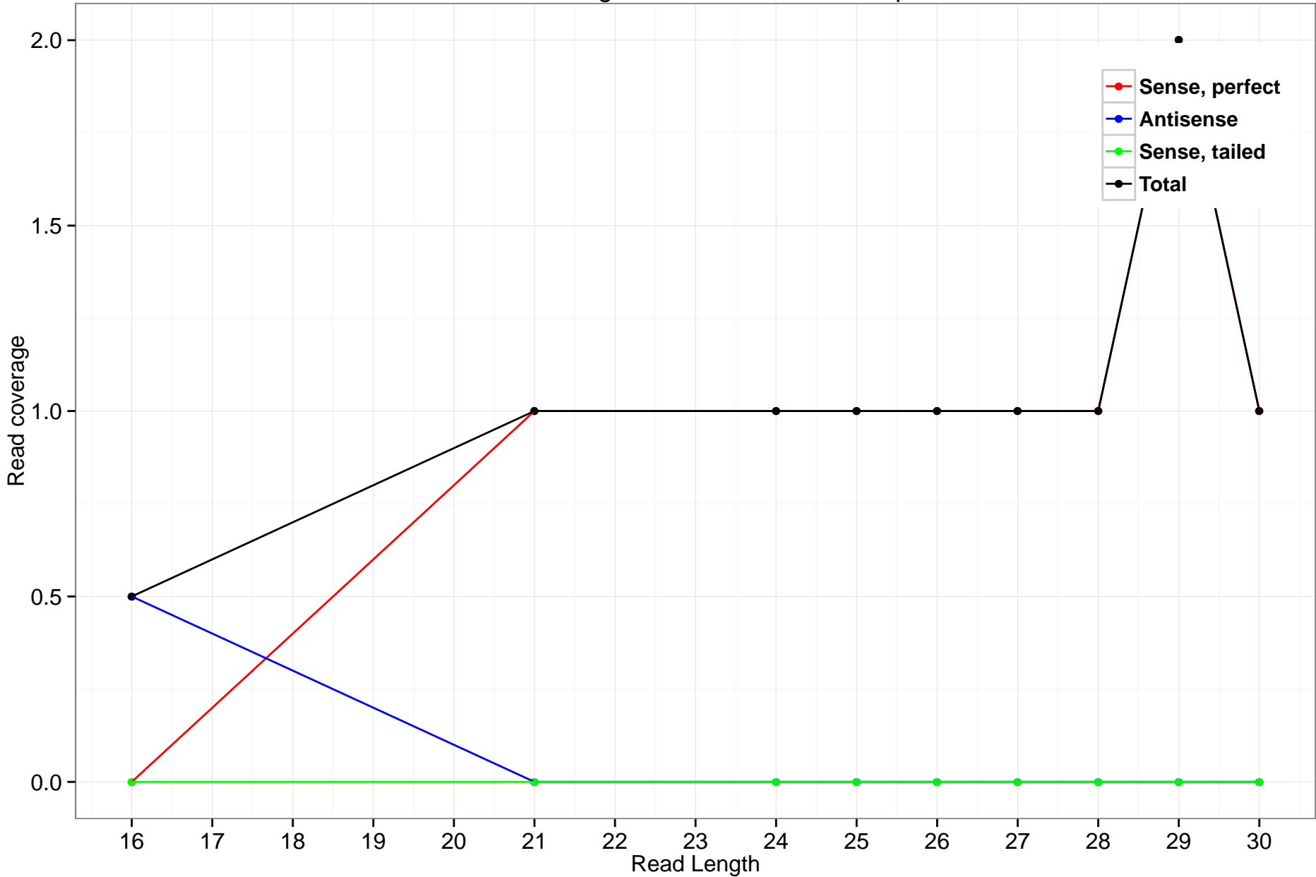
rheMac3_genscan_chr10.1173_2.5p
