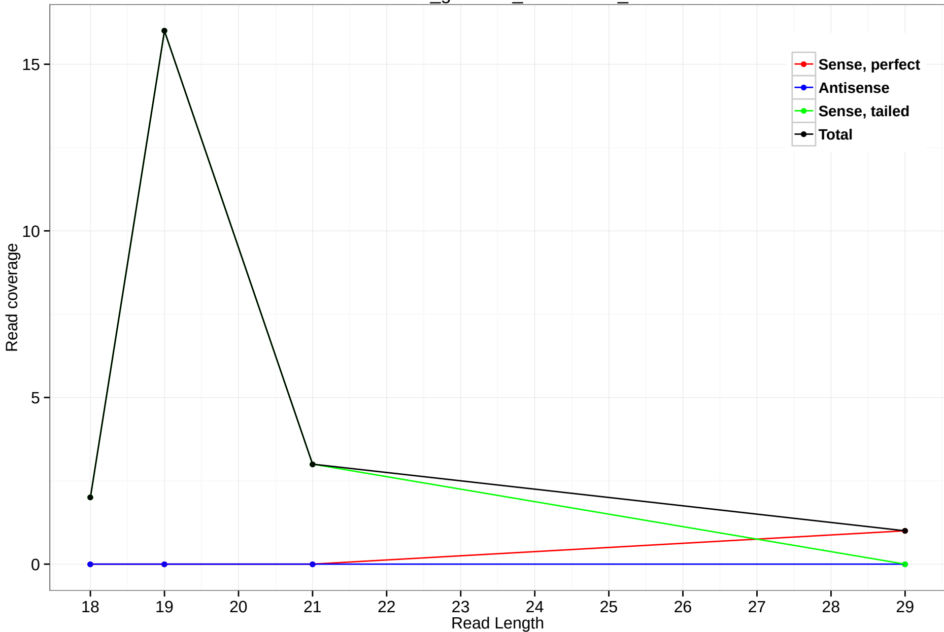
rheMac3_genscan_chr10.1047_0
