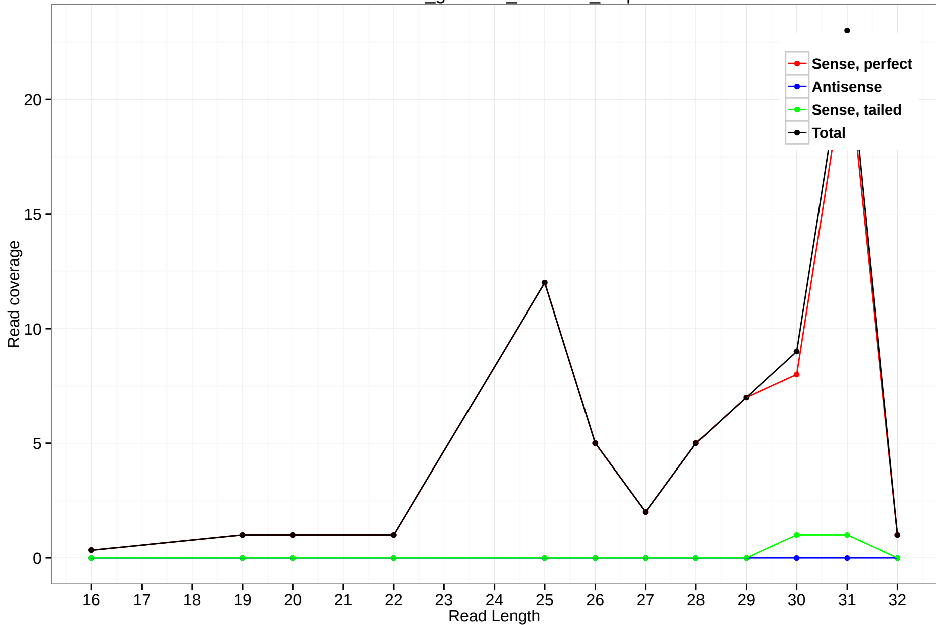
rheMac3_genscan_chr1.979_2.5p
