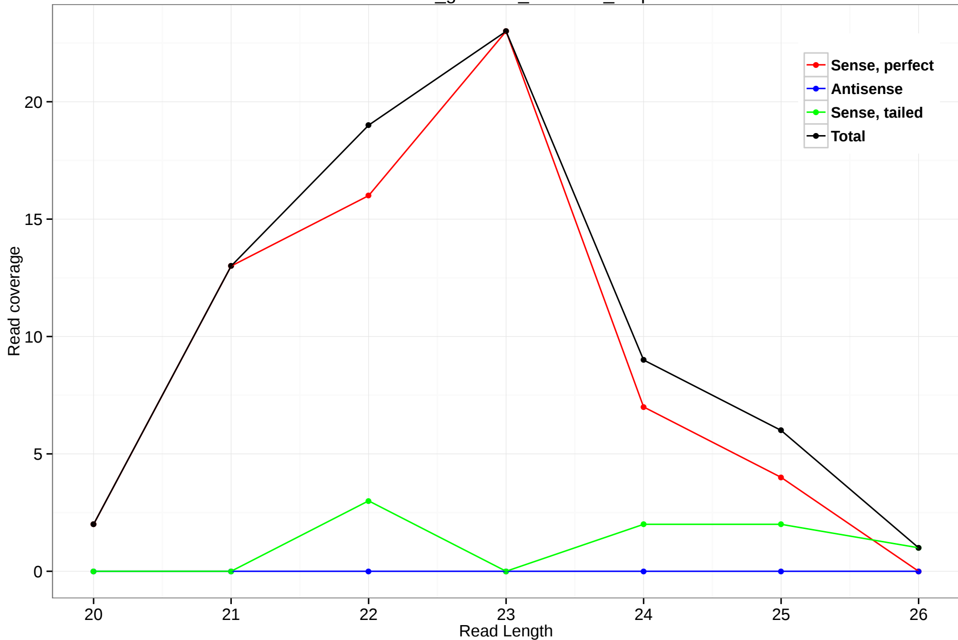
rheMac3_genscan_chr1.950_8.3p
