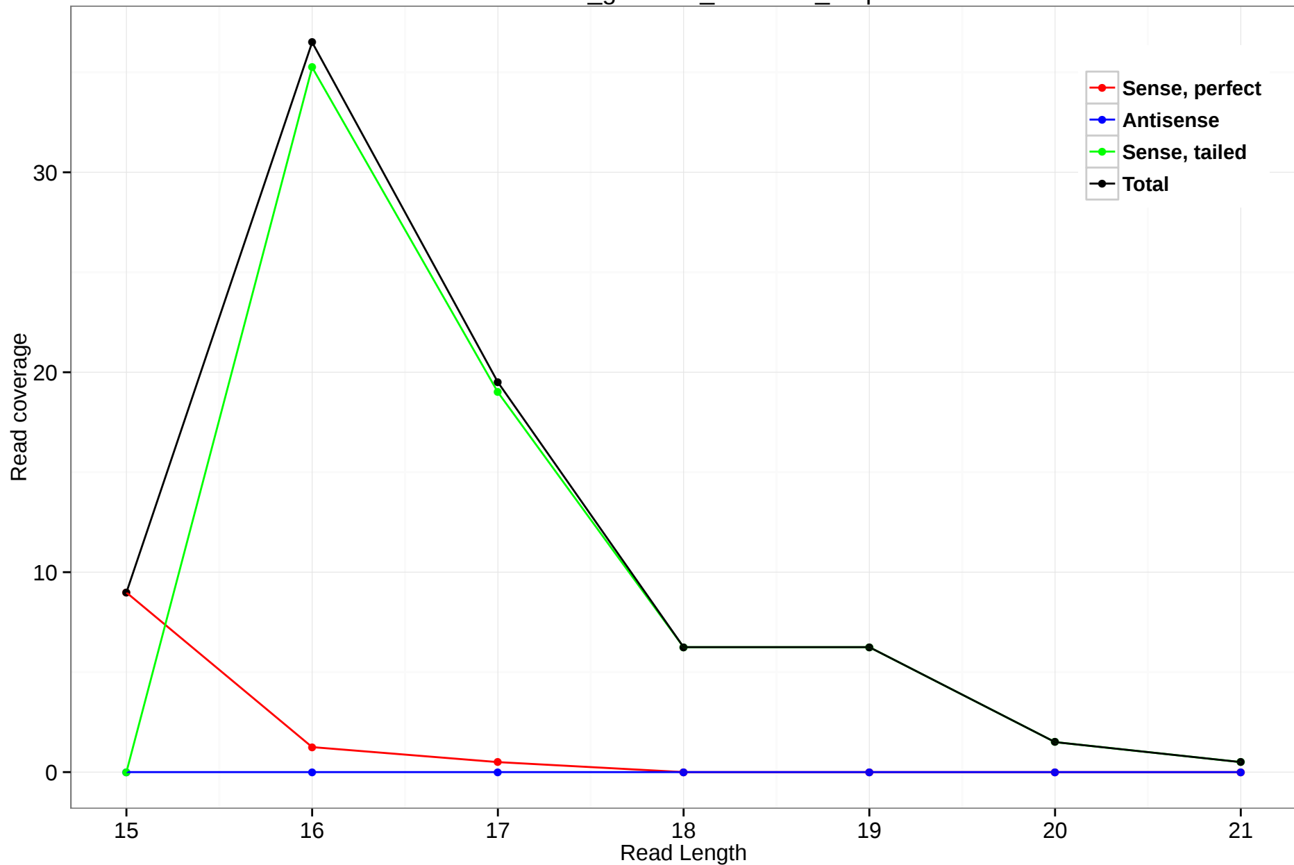
rheMac3_genscan_chr1.946_3.3p
