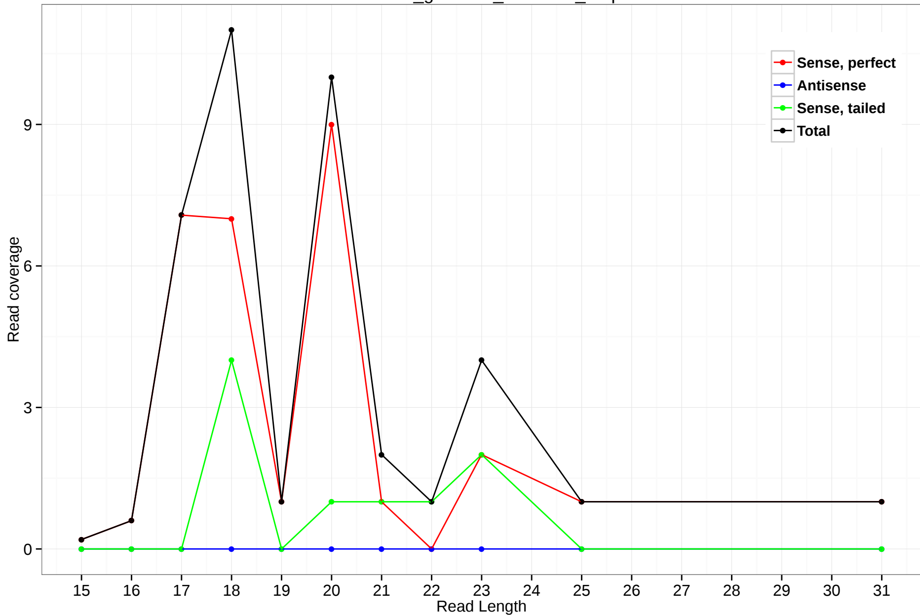
rheMac3_genscan_chr1.946_0.5p
