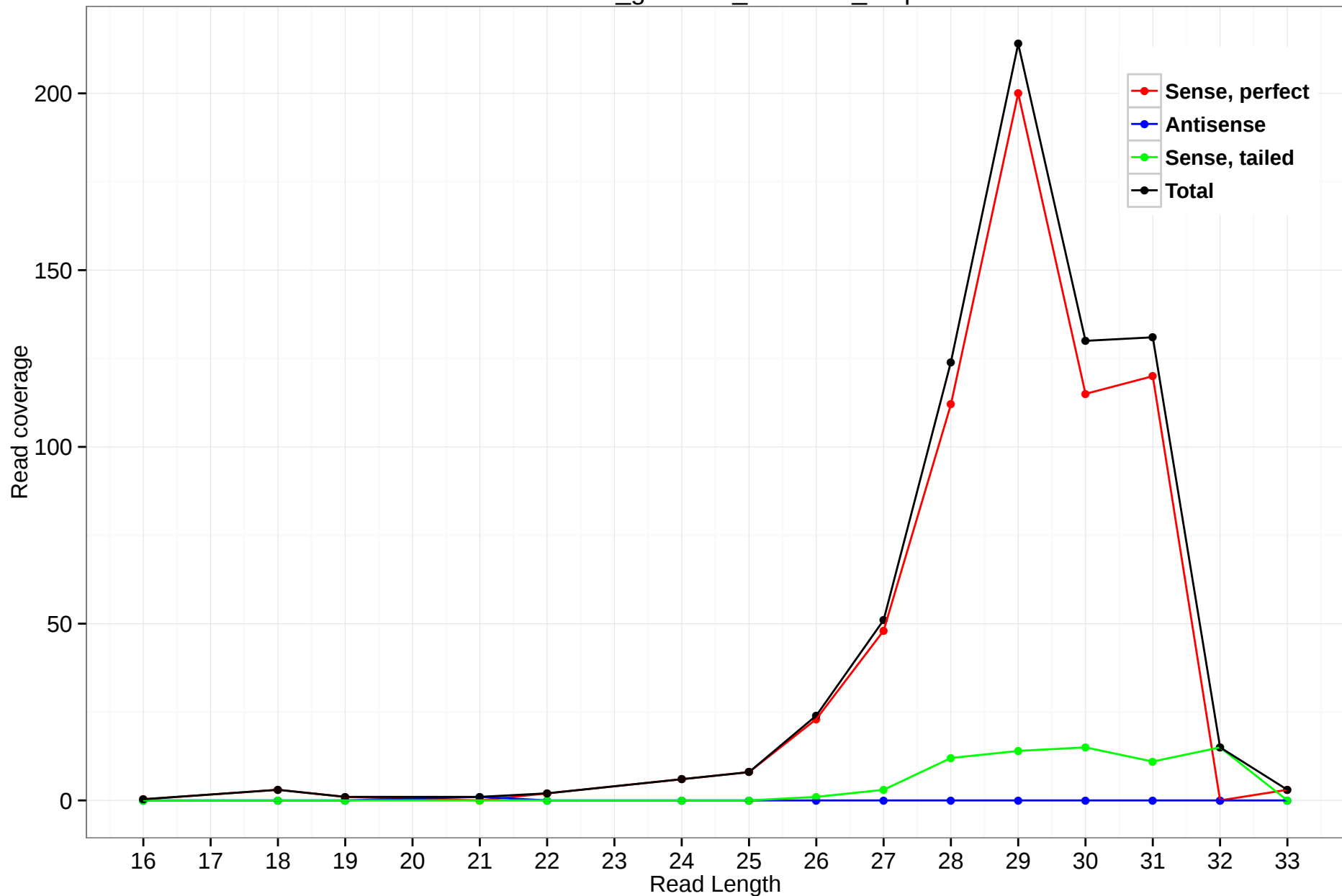
rheMac3_genscan_chr1.907_9.3p
