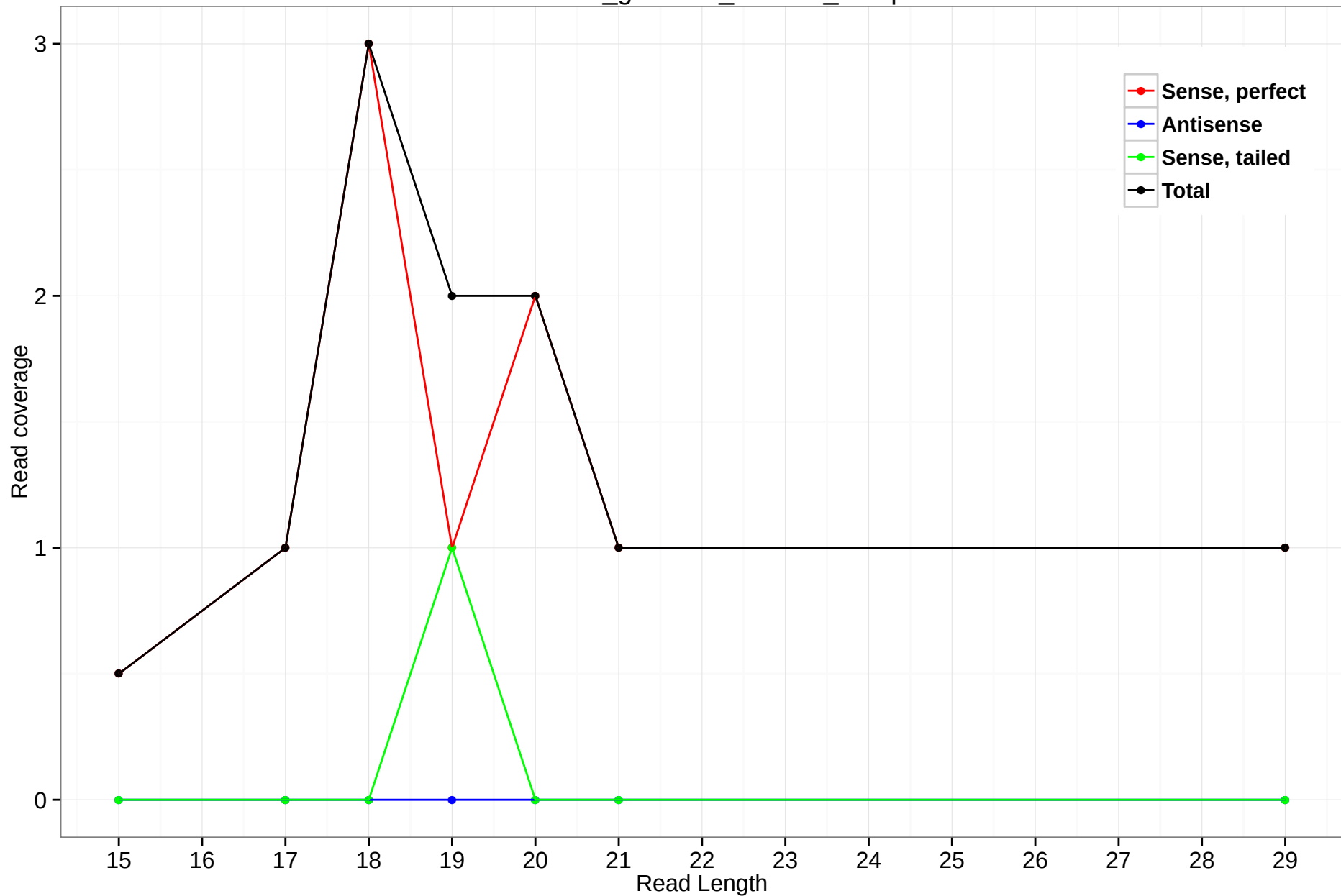
rheMac3_genscan_chr1.89_35.5p
