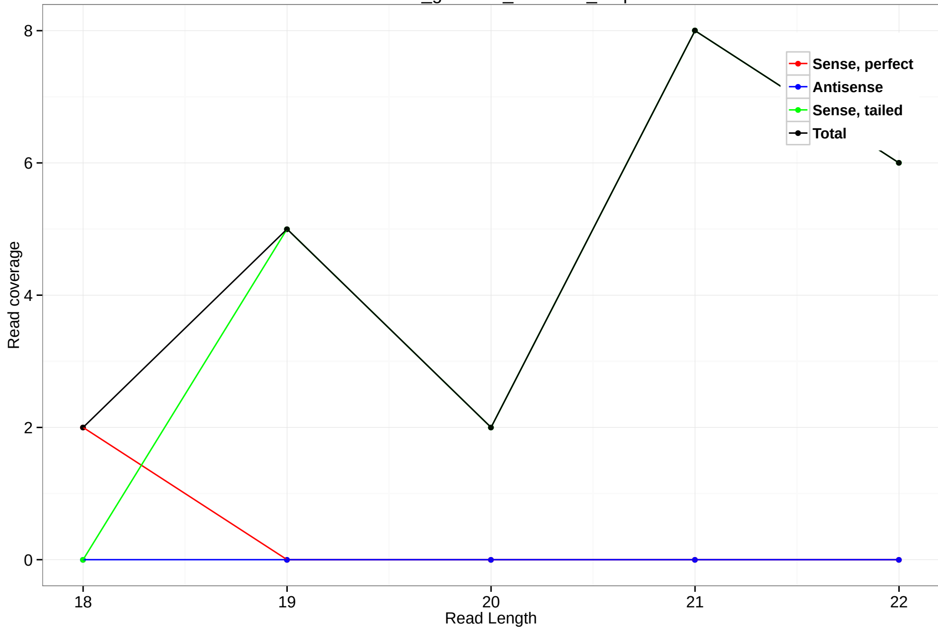
rheMac3_genscan_chr1.870_1.5p
