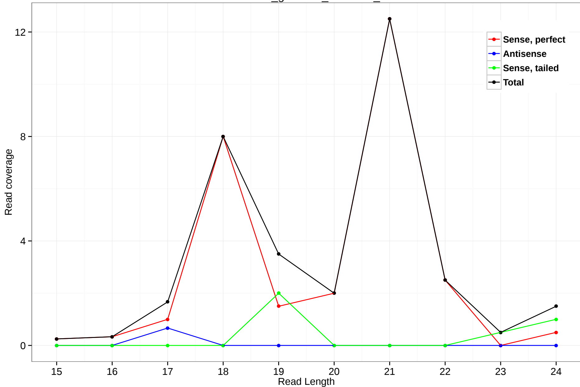
rheMac3_genscan_chr1.846_1
