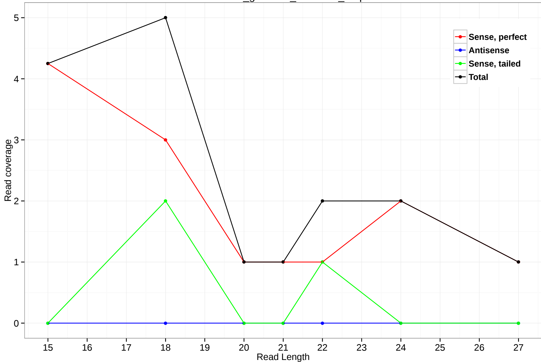
rheMac3_genscan_chr1.844_0.5p
