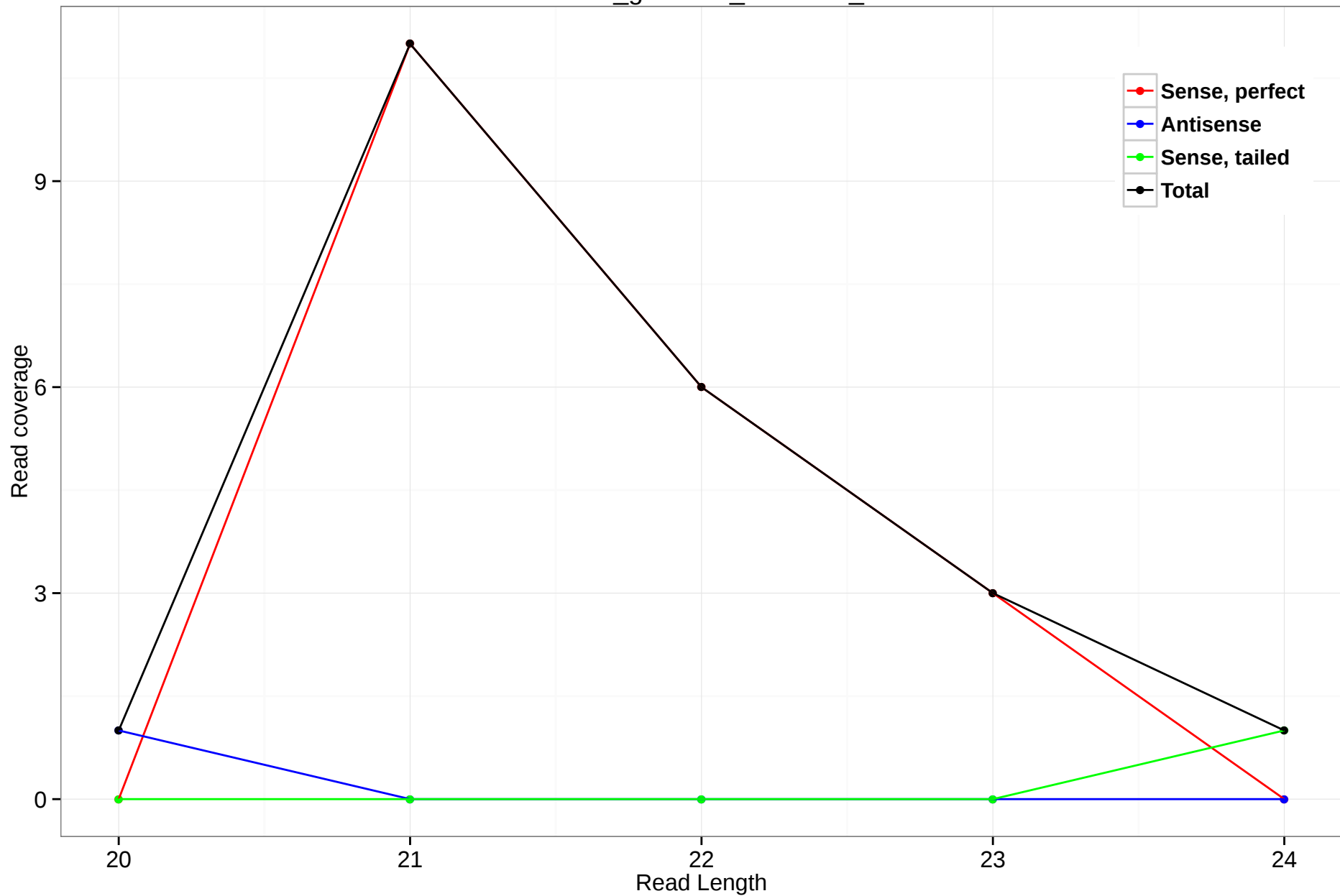
rheMac3_genscan_chr1.809_18
