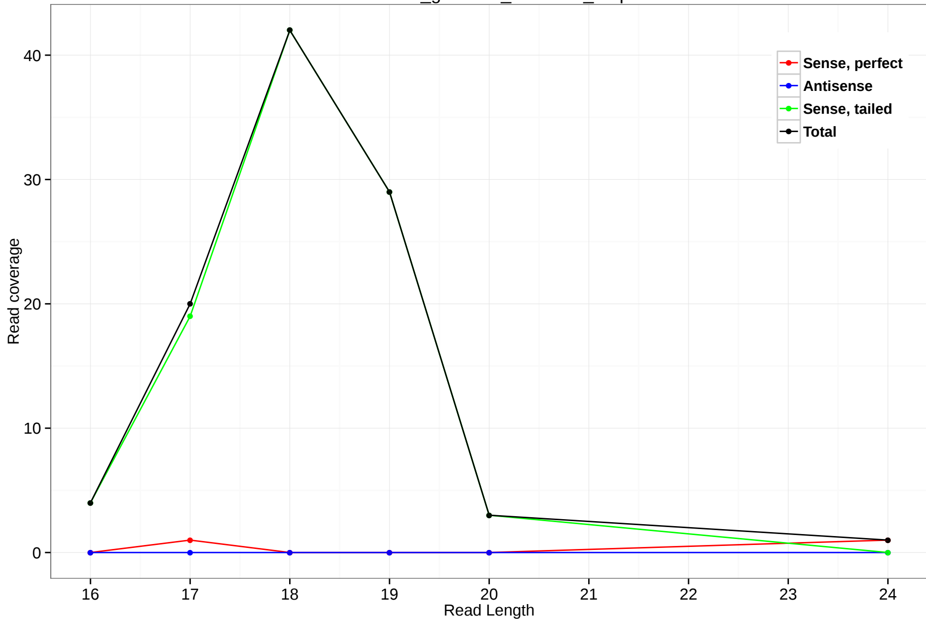
rheMac3_genscan_chr1.804_3.5p
