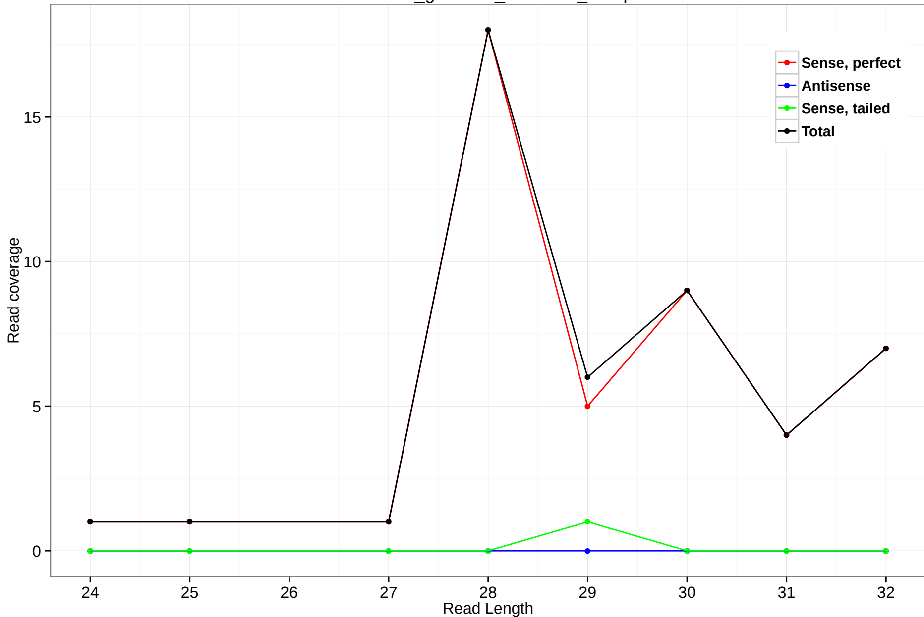
rheMac3_genscan_chr1.796_18.5p
