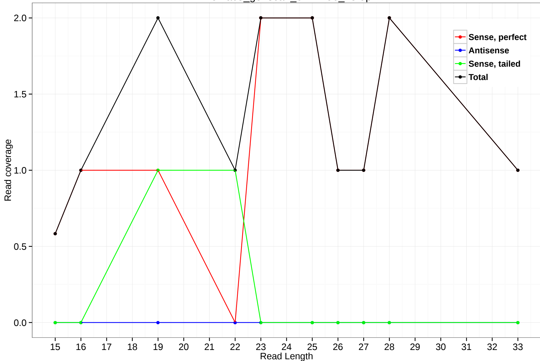
rheMac3_genscan_chr1.796_15.5p
