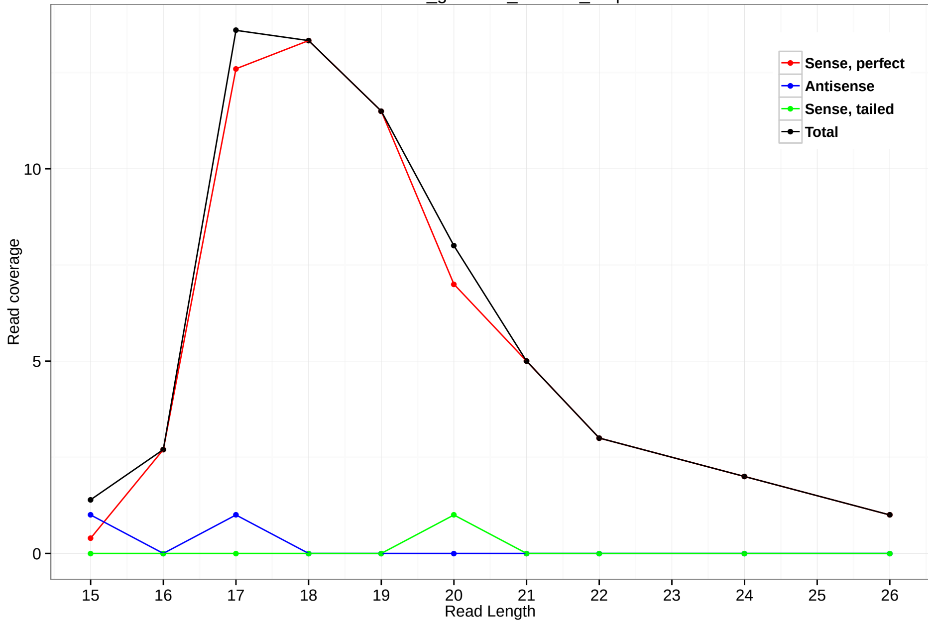
rheMac3_genscan_chr1.78_5.5p
