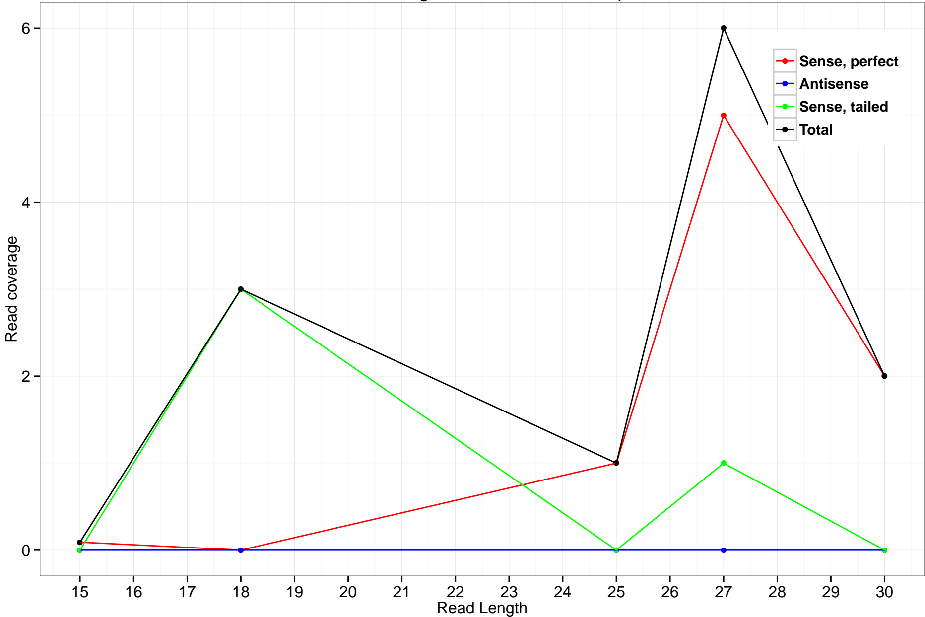
rheMac3_genscan_chr1.776_47.5p
