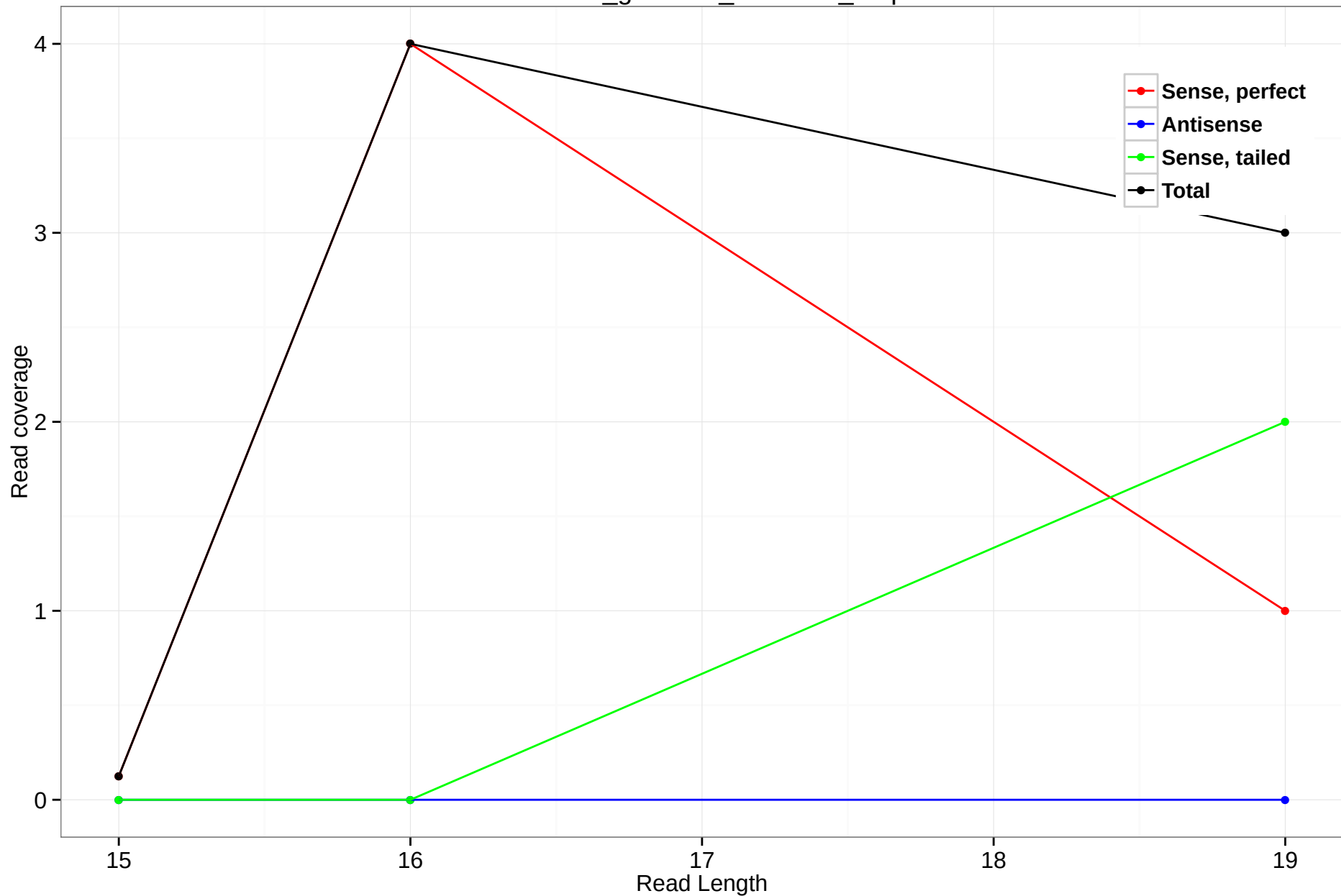
rheMac3_genscan_chr1.773_1.3p
