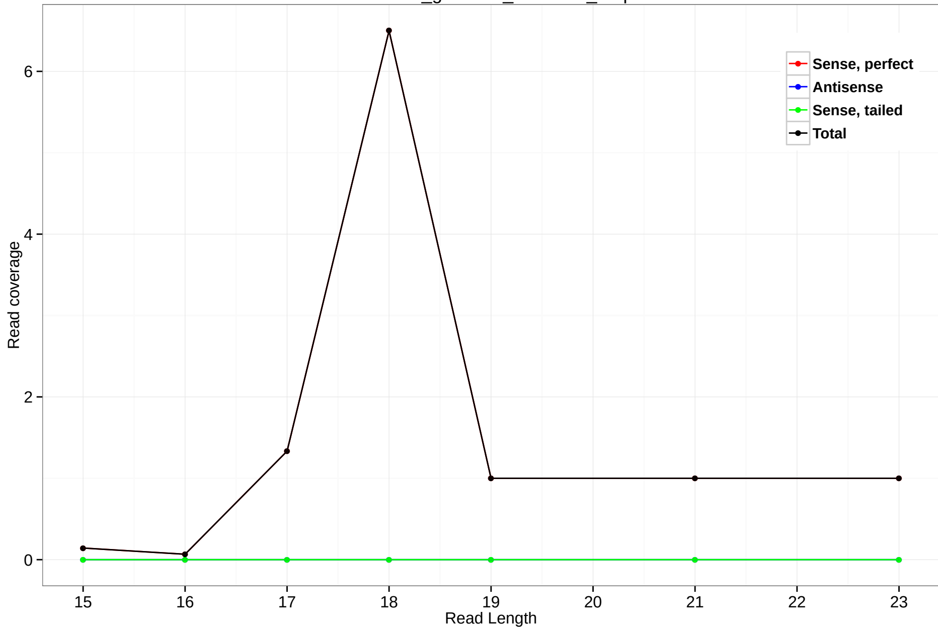
rheMac3_genscan_chr1.764_3.3p
