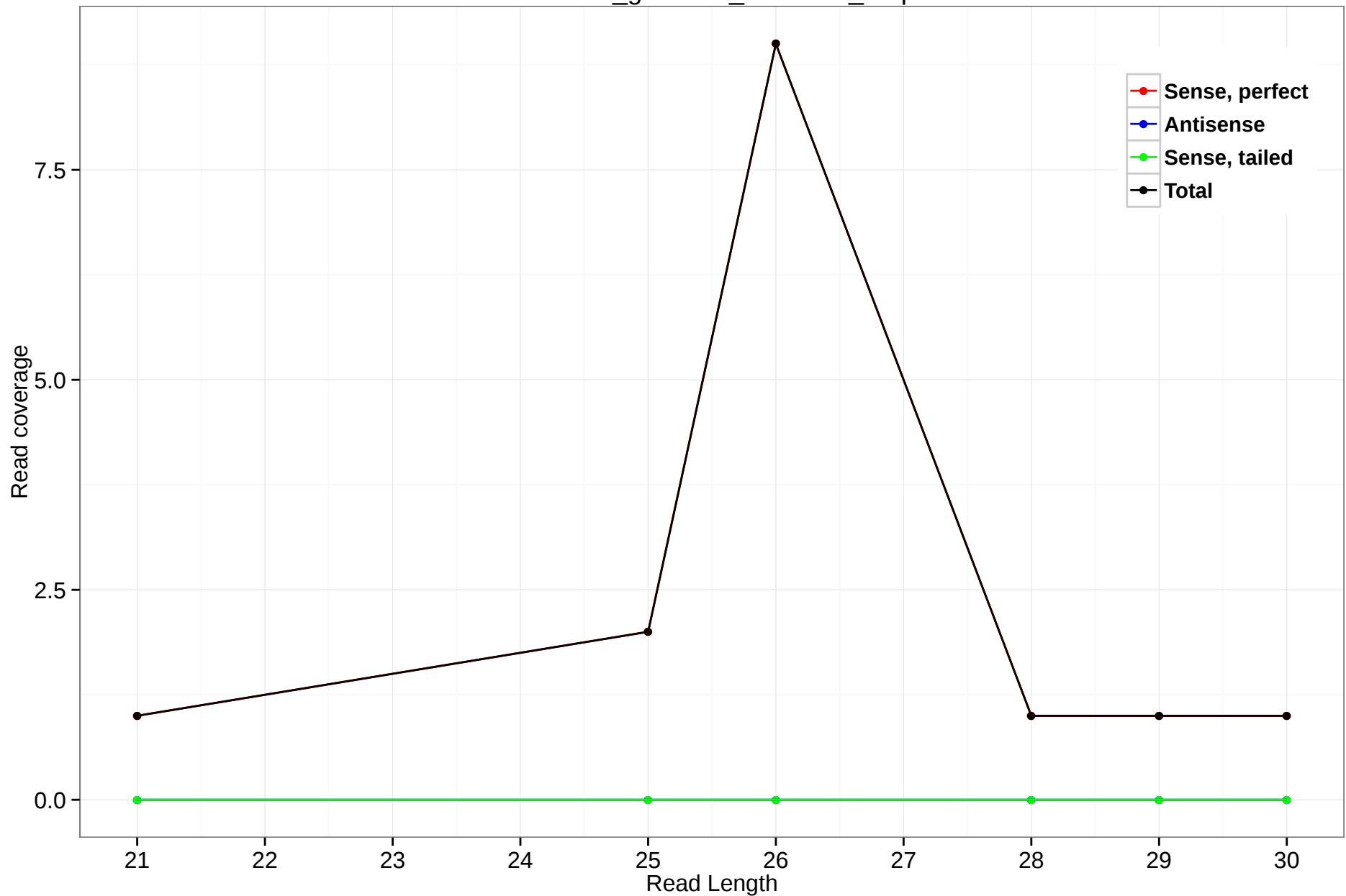
rheMac3_genscan_chr1.740_3.5p
