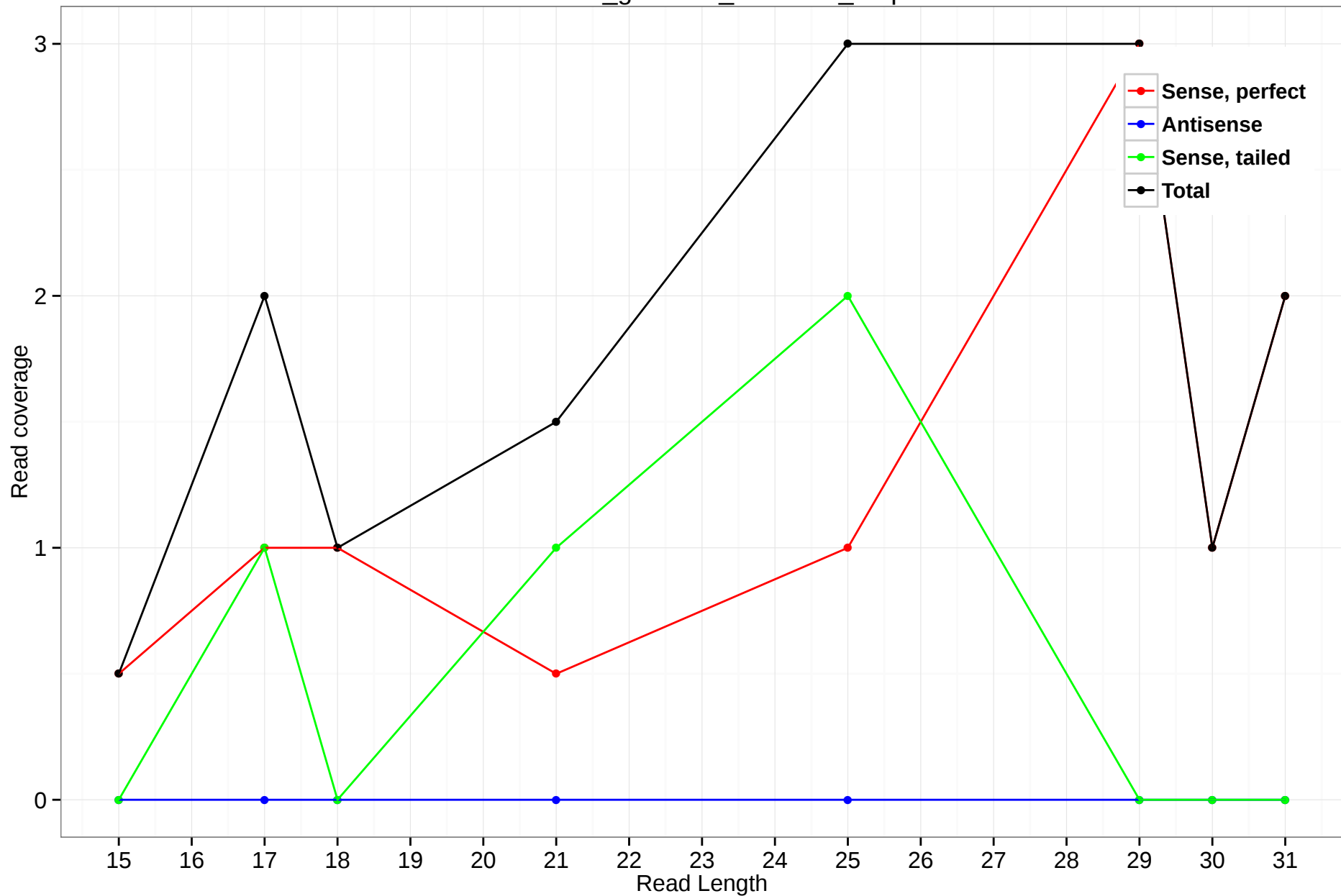
rheMac3_genscan_chr1.733_2.5p
