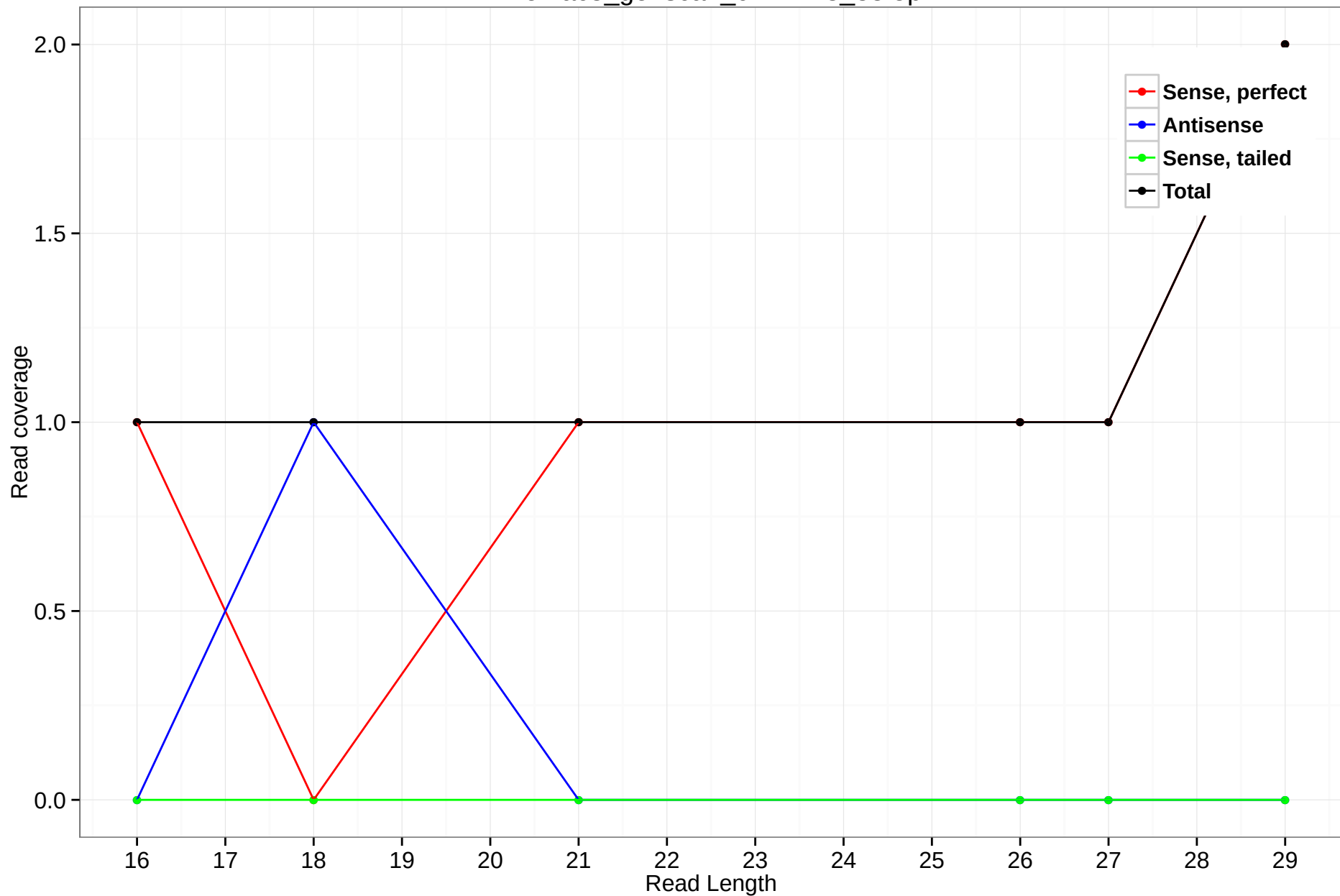
rheMac3_genscan_chr1.728_33.5p
