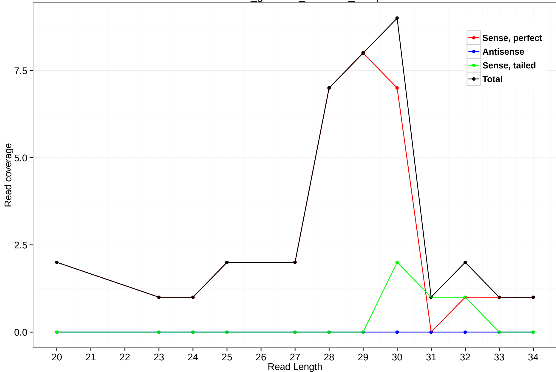
rheMac3_genscan_chr1.728_21.3p
