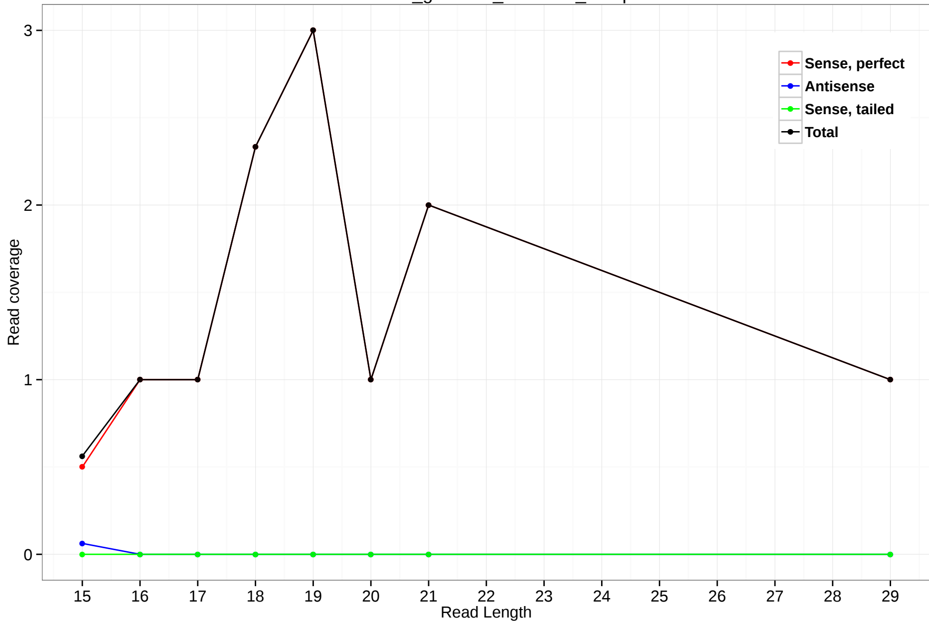
rheMac3_genscan_chr1.725_32.3p
