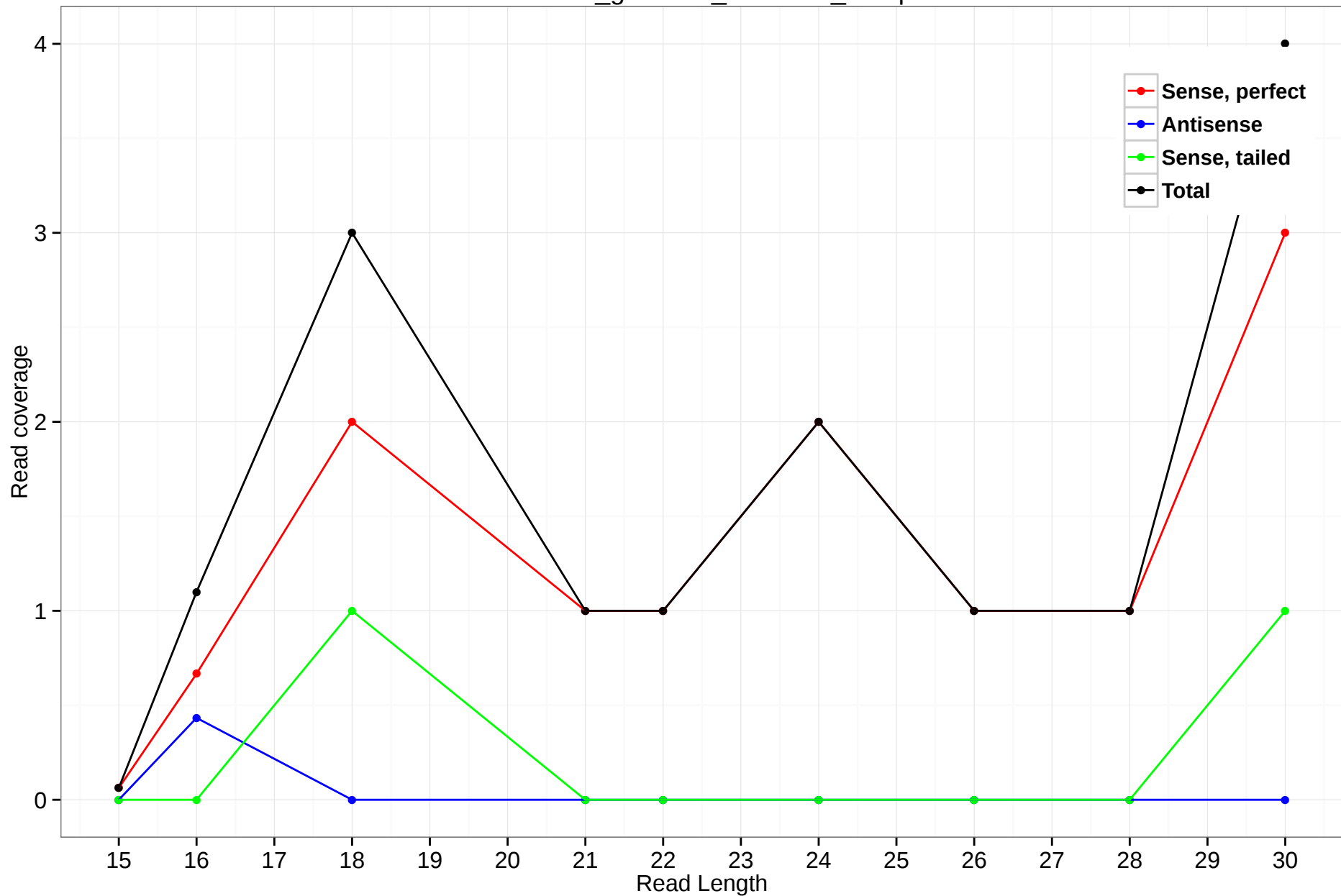
rheMac3_genscan_chr1.692_14.5p
