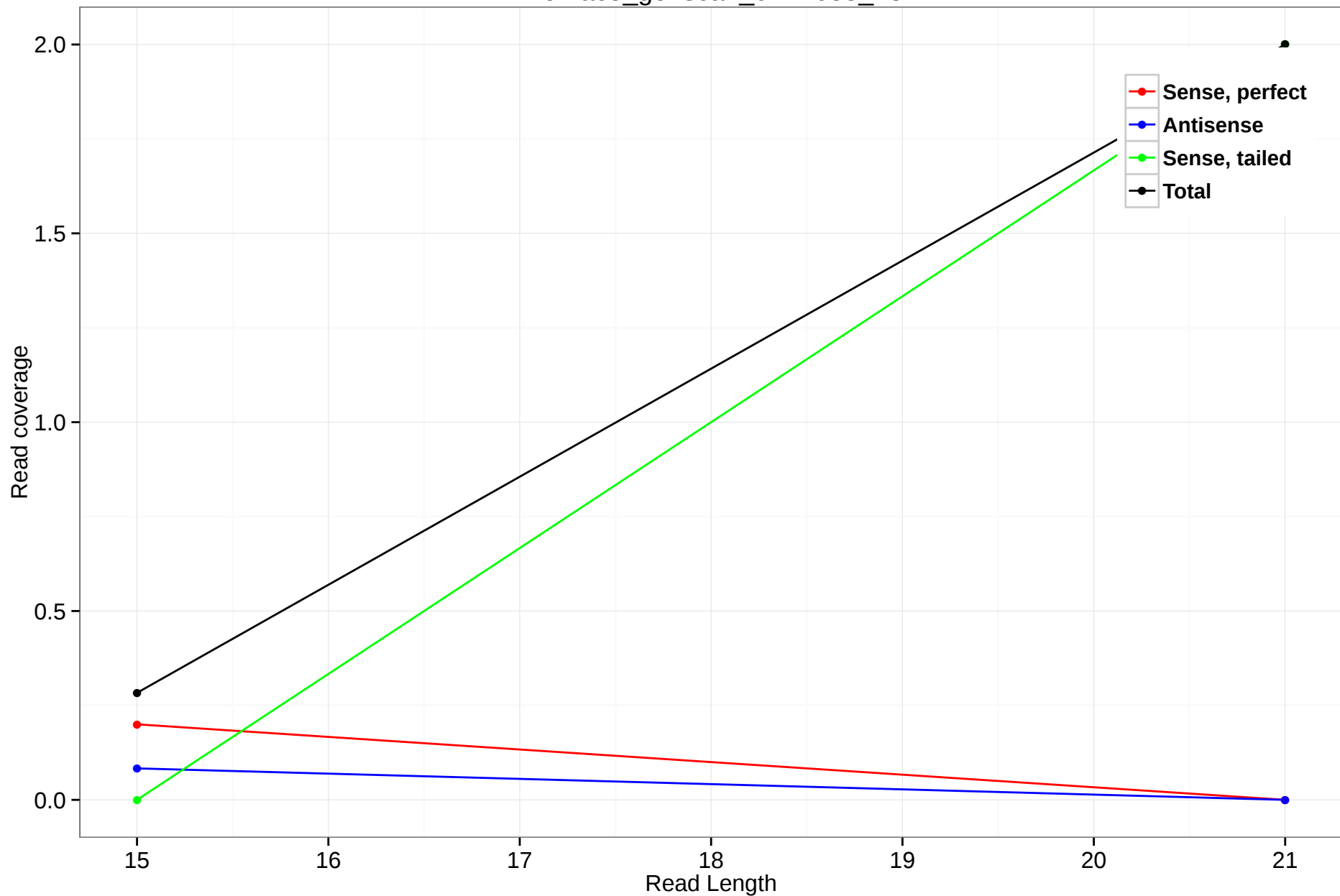
rheMac3_genscan_chr1.685_43
