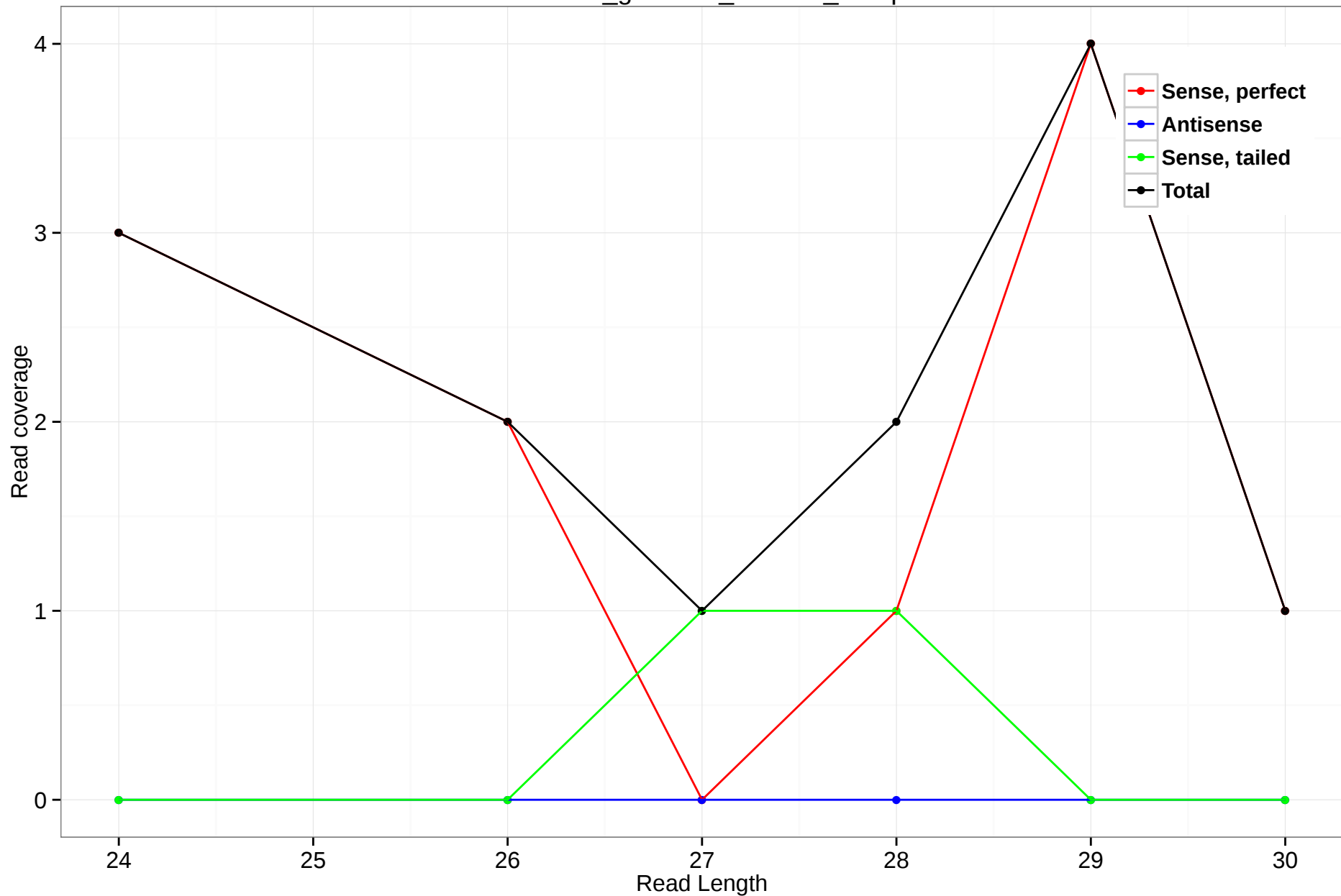
rheMac3_genscan_chr1.67_17.3p
