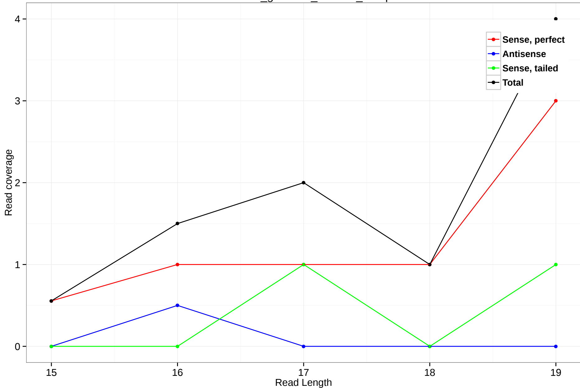
rheMac3_genscan_chr1.67_12.5p
