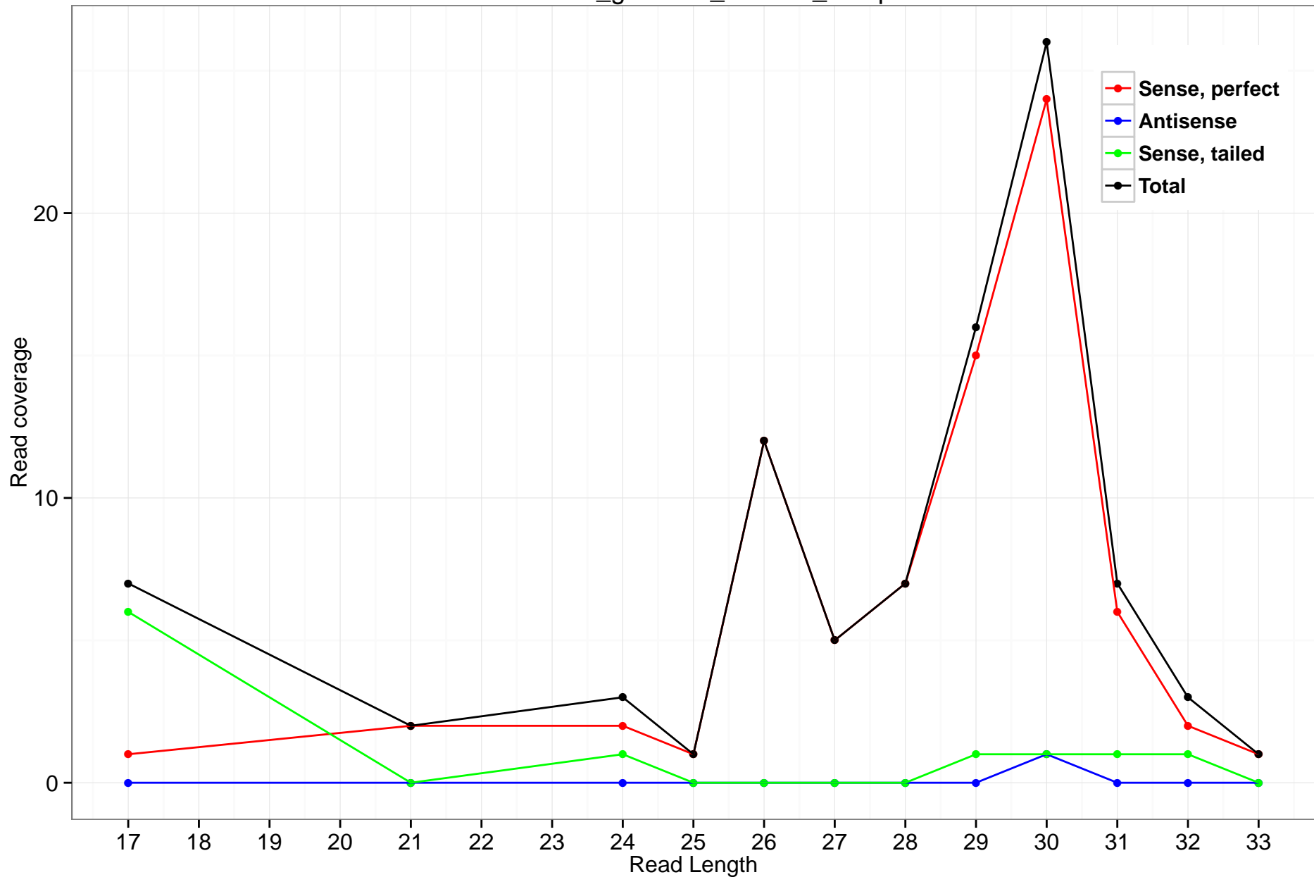
rheMac3_genscan_chr1.66_14.3p
