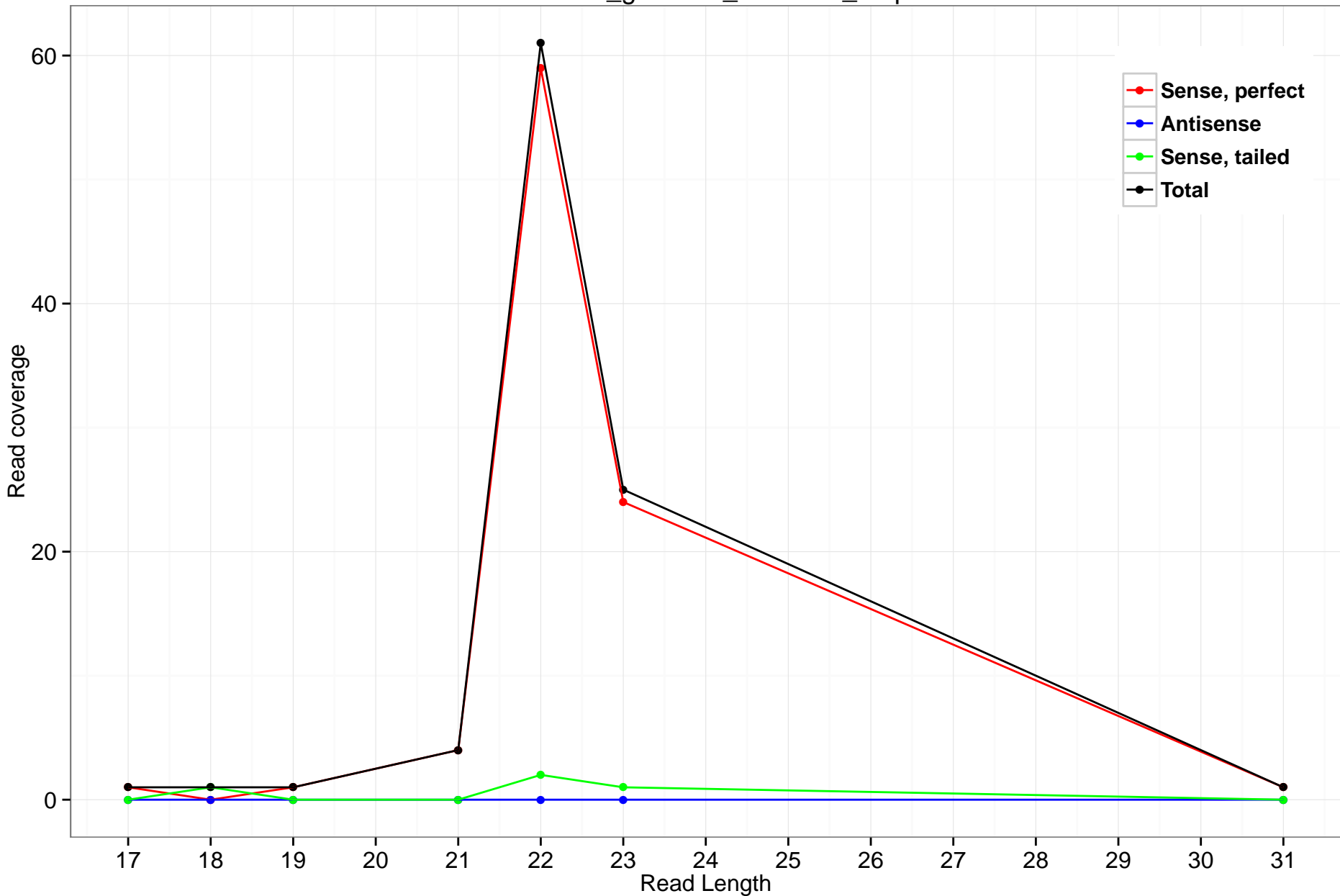
rheMac3_genscan_chr1.663_0.3p
