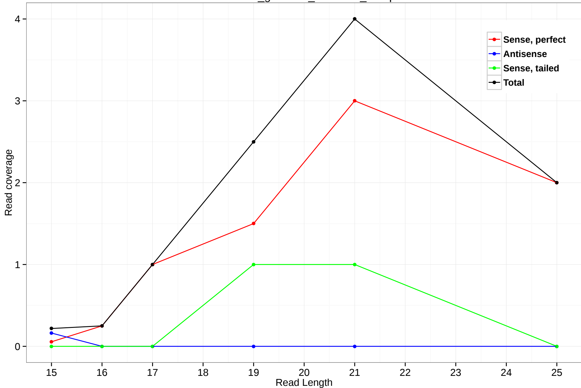
rheMac3_genscan_chr1.662_25.3p
