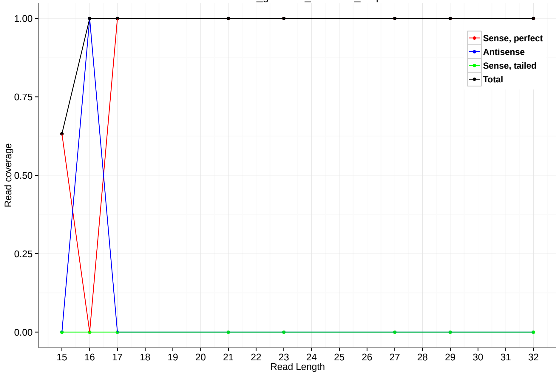
rheMac3_genscan_chr1.631_2.5p
