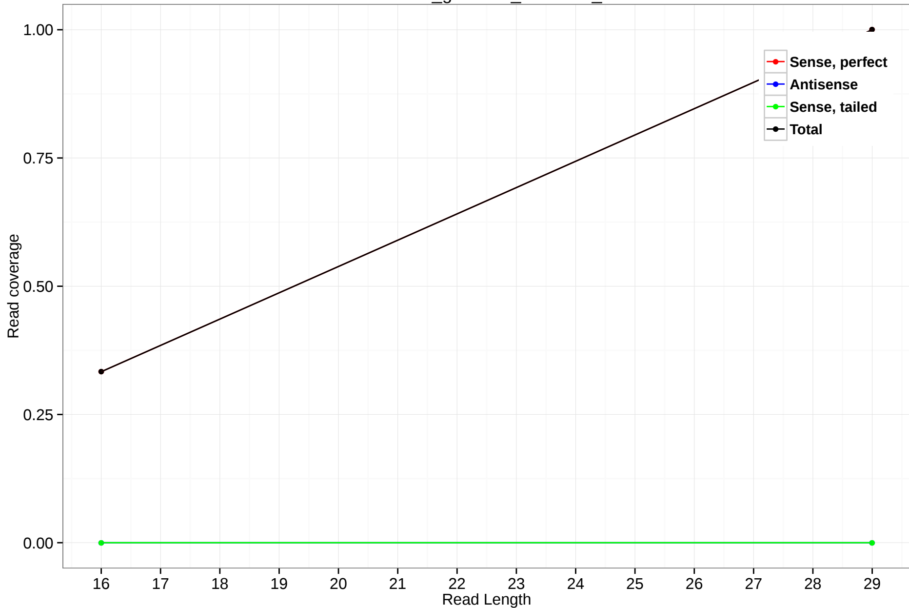
rheMac3_genscan_chr1.570_4
