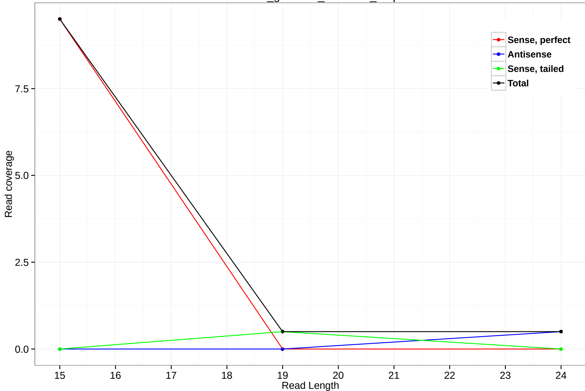
rheMac3_genscan_chr1.532_3.5p
