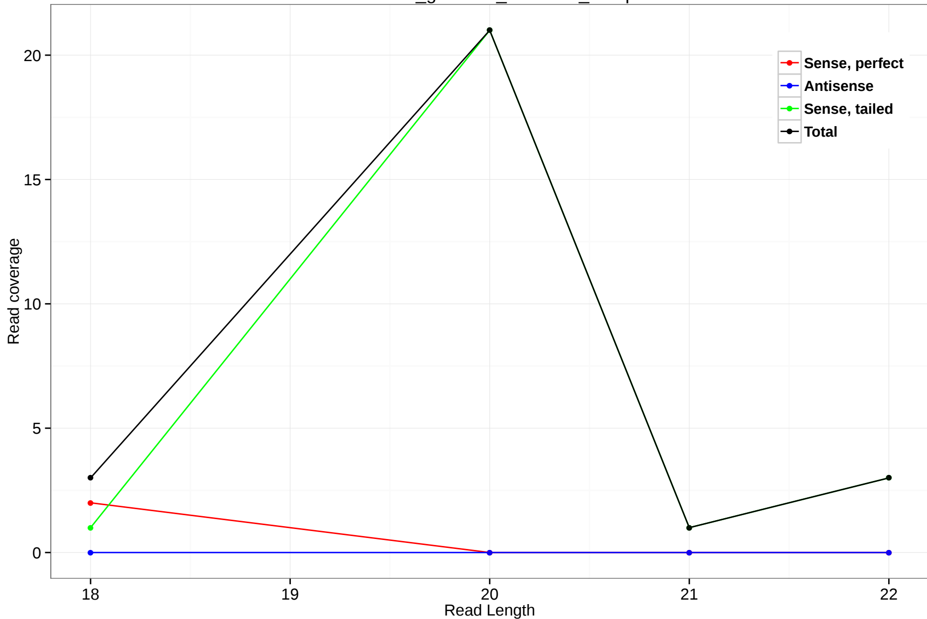
rheMac3_genscan_chr1.469_45.5p
