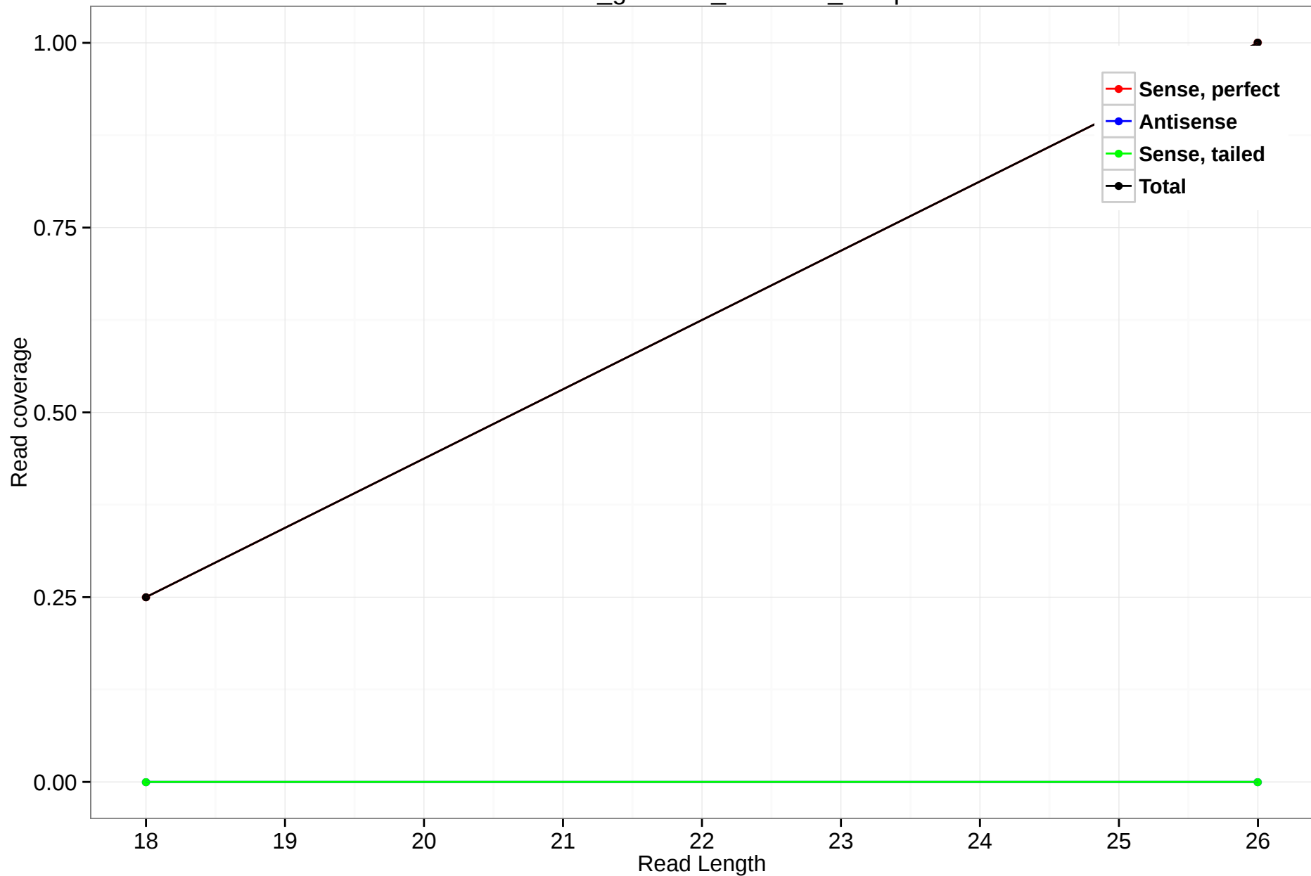
rheMac3_genscan_chr1.468_30.3p
