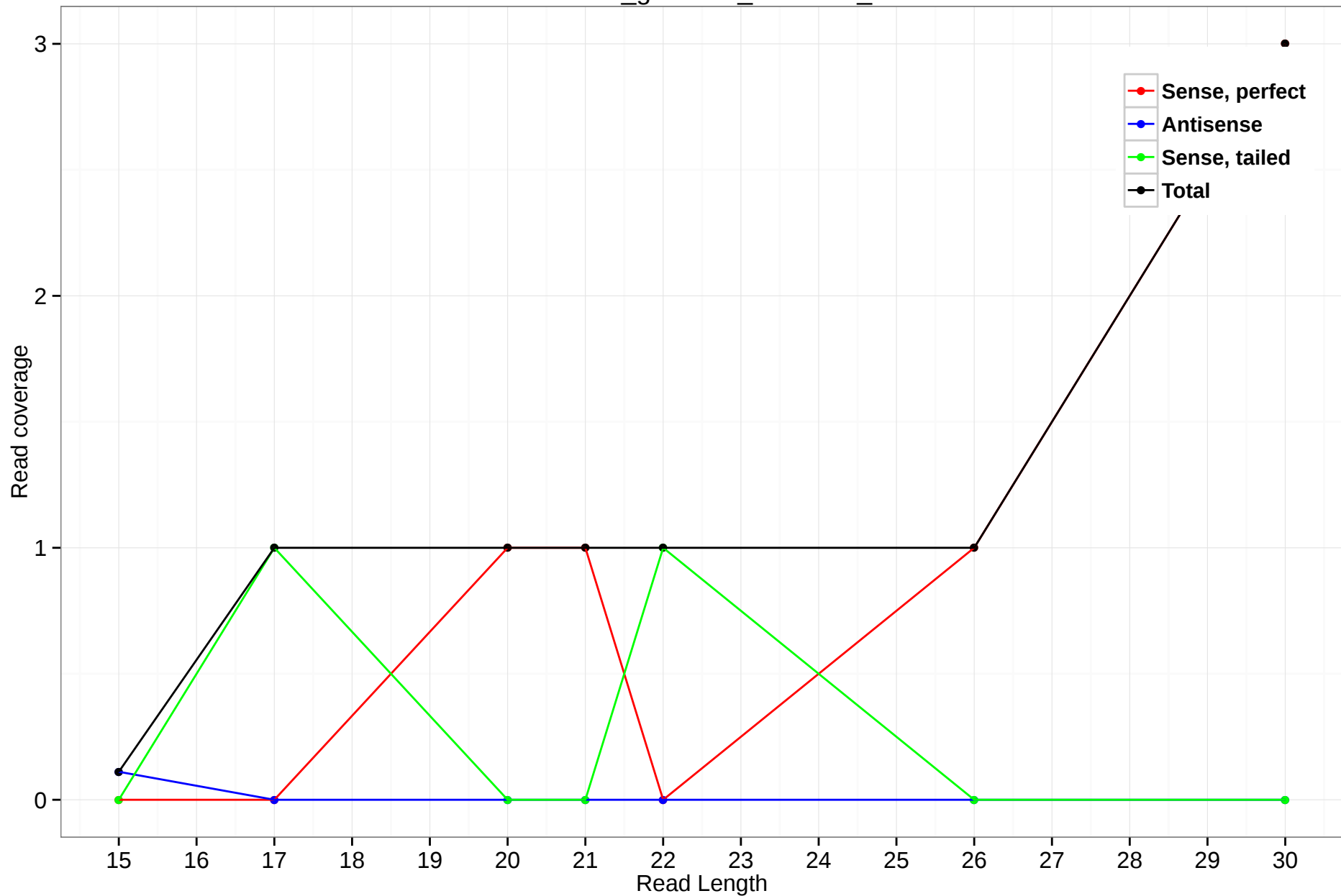
rheMac3_genscan_chr1.468_2
