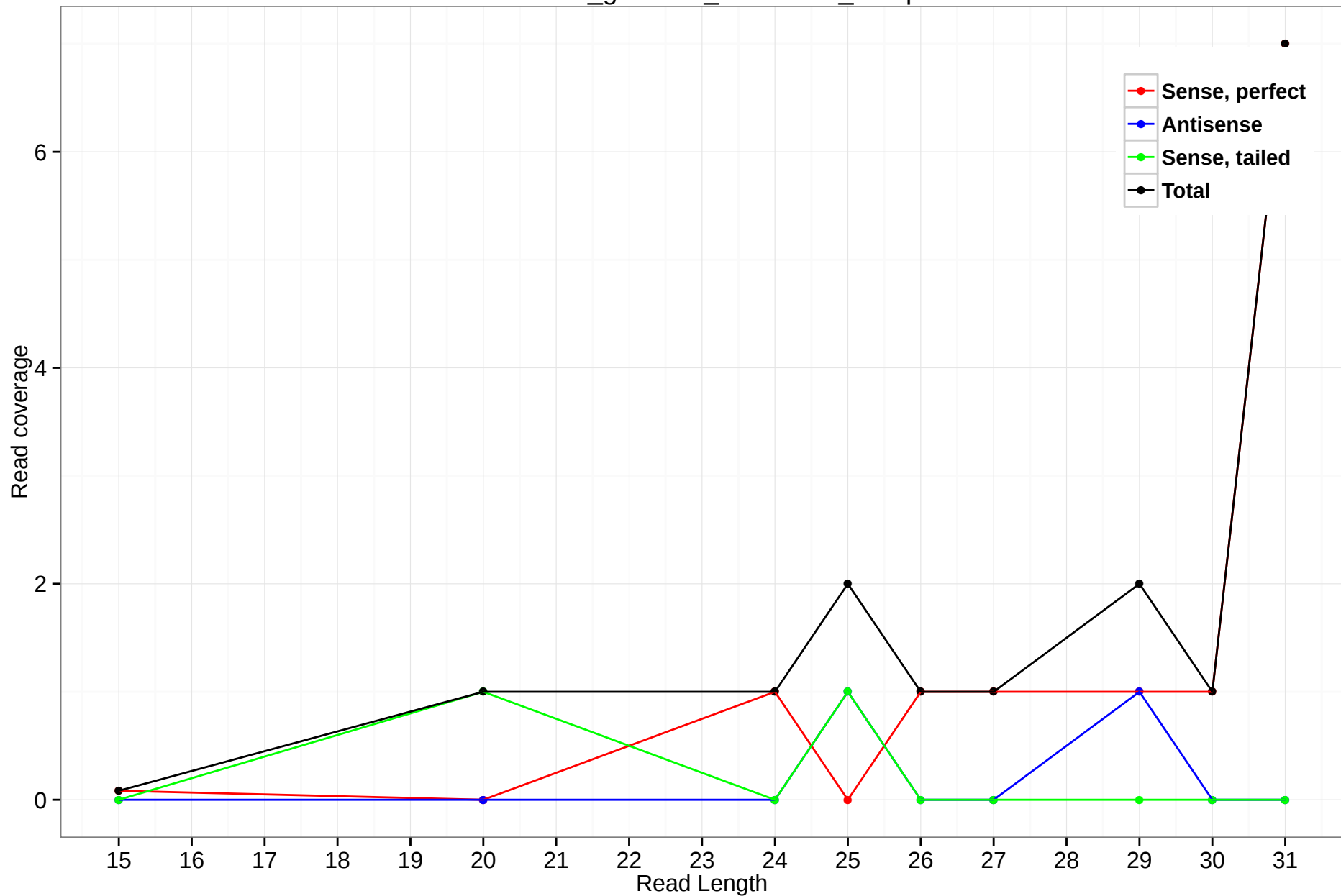
rheMac3_genscan_chr1.4681_13.5p
