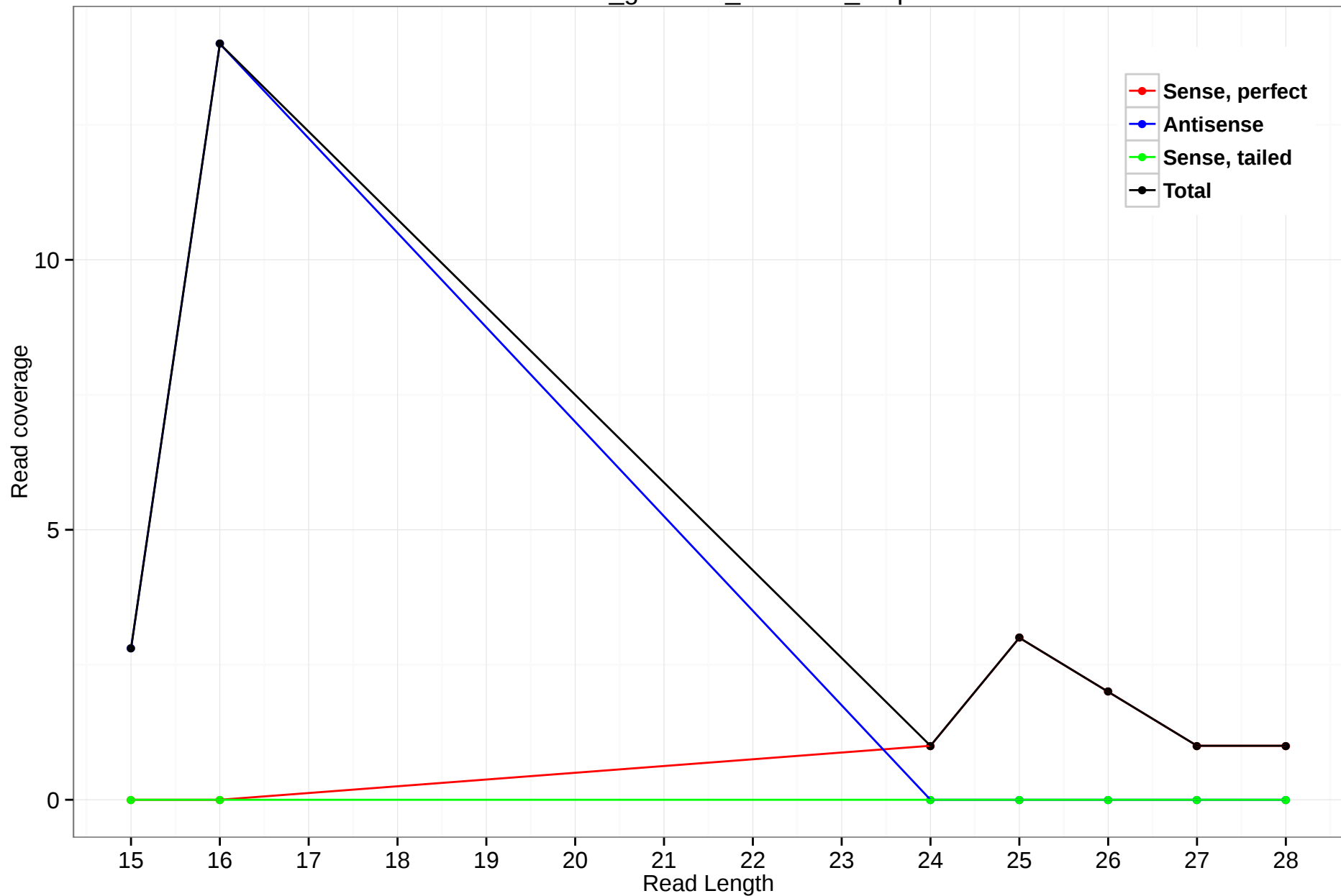
rheMac3_genscan_chr1.465_2.3p
